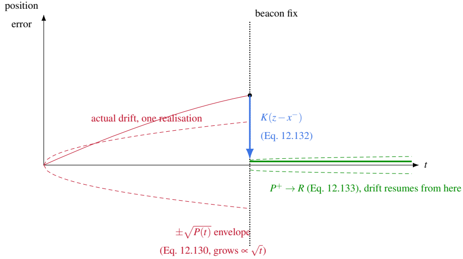
Figure 12.30: The predicted shape of the straight-line experiment (§12.20.3), derived, not measured: an uncertainty envelope opening as \sqrt{t} while no fix arrives (dashed red), an abrupt correction sized by the innovation at the instant a fix lands (blue arrow, Eq. 12.132), and a tight, beacon-precision envelope resuming immediately after (dashed green). No data from this rover appears in this figure; it is what Eq. 12.130–12.133 require, against which a real run can be checked.
