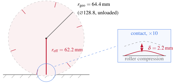
Figure 12.31: The 2.2 mm of Eq. 12.134 drawn to scale on the wheel, where it is invisible, and again at \times 10 , where it is not. That ratio is the whole reason this quantity is easy to leave wrong in a configuration file for months.
