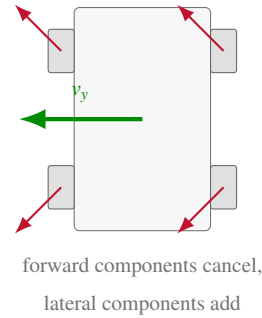
Figure 12.33: Left: the roller diagonals in the X pattern, with the two geometric lengths of Eq. 12.142. Right: the second degenerate case of Eq. 12.143 — four diagonal wheel forces whose longitudinal parts cancel in pairs, leaving a pure v_y .
