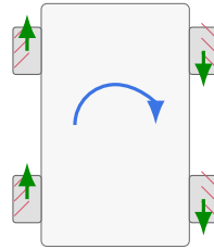
Mecanum — rolling
