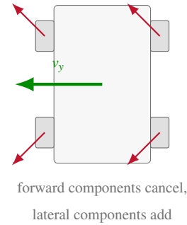
Figure 12.33: Left: the roller diagonals in the X pattern, with the two geometric lengths of Eq. 12.138. Right: the second degenerate case of Eq. 12.139 — four diagonal wheel forces whose longitudinal parts cancel in pairs, leaving a pure v_y .
