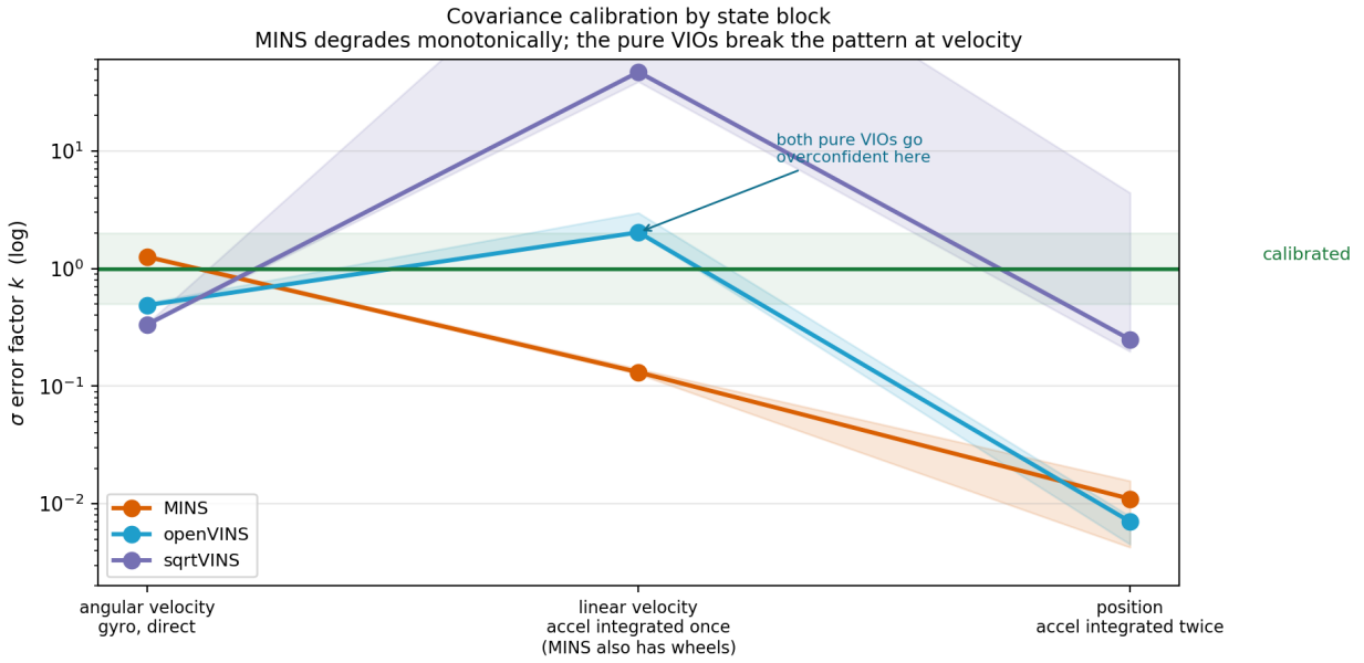
Figure 11.7: The \sigma error factor k of Eq. (11.9) for each state block, medians across the three stationary recordings with the shaded band giving their spread. Unity is calibrated. MINS declines monotonically from the directly measured angular rate to the twice-integrated position. The two pure VIO filters do not: both are overconfident precisely at linear velocity, the one channel for which MINS carries an independent measurement.
