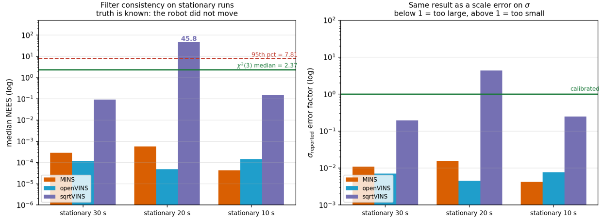
Figure 11.5: Consistency on the three stationary recordings, where the true position is known exactly. Left: median NEES, logarithmic, against the \chi^2(3) median of 2.37 (solid) and its 95th percentile of 7.81 (dashed). MINS and openVINS sit four orders of magnitude below the reference; sqrtVINS exceeds the 95th percentile on one run. Right: the same result expressed by Eq. (11.9) as a multiplicative error on the reported \sigma , where unity is calibrated.
