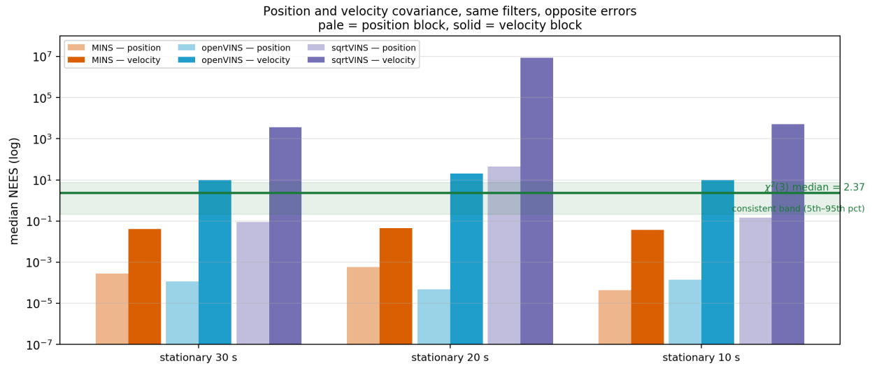
Figure 11.6: The two covariance blocks of each filter, on the same recordings. Pale bars are the position block, solid bars the velocity block; the green band spans the 5th to 95th percentiles of \chi^2(3) , within which a consistent filter should fall. MINS sits below it on both blocks, closer on velocity. openVINS falls far below on position and above on velocity — the same matrix wrong in opposite directions. sqrtVINS leaves the plot.
