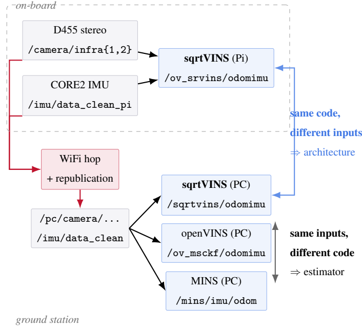
Figure 12.39: The two data paths, and why the ground instance of sqrtVINS is retained even though it is redundant as an estimator. Holding one of the two factors fixed at a time is what makes the decomposition (12.184) available.
