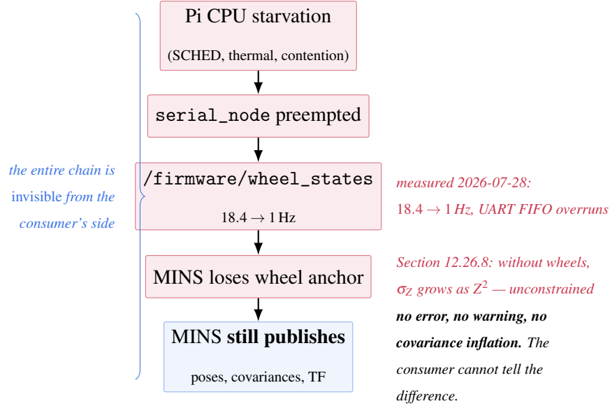
Figure 12.37: The blind spot that motivates external instrumentation. Each arrow is a mechanism verified on this platform; the terminal state is indistinguishable from nominal operation for any node downstream of MINS. A monitor placed outside the chain is the only way to detect it.
