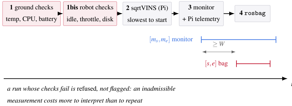
Figure 12.40: Campaign sequence. Stages 1 and 1bis are vetoes. The monitor’s support strictly contains the recording’s, with at least one window W of lead so that its sliding estimators are converged before the first message is written — condition (12.190).
