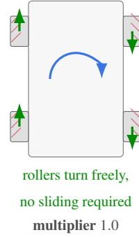
Mecanum — rolling
