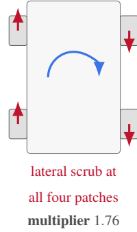
Standard — skid-steer
