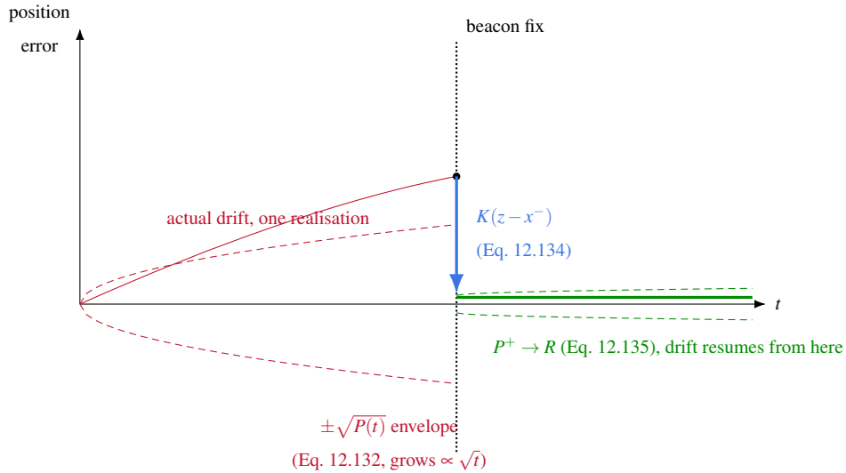
Figure 12.30: The predicted shape of the straight-line experiment (§12.21.3), derived, not measured: an uncertainty envelope opening as \sqrt{t} while no fix arrives (dashed red), an abrupt correction sized by the innovation at the instant a fix lands (blue arrow, Eq. 12.134), and a tight, beacon-precision envelope resuming immediately after (dashed green). No data from this rover appears in this figure; it is what Eq. 12.132–12.135 require, against which a real run can be checked.
