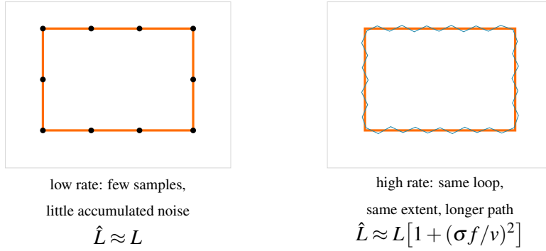
Figure 12.17: Why cumulative path length must not be compared across sampling rates. Both panels show the same physical loop with the same spatial extent; the right-hand estimator merely samples it faster. Every additional sample contributes its own noise excursion, so the measured path lengthens quadratically in the sampling rate (Eq. 12.85) while the extent is inflated only by the additive constant of Eq. 12.83. The two ratios quoted in Fig. 12.11 differ for exactly this reason.
