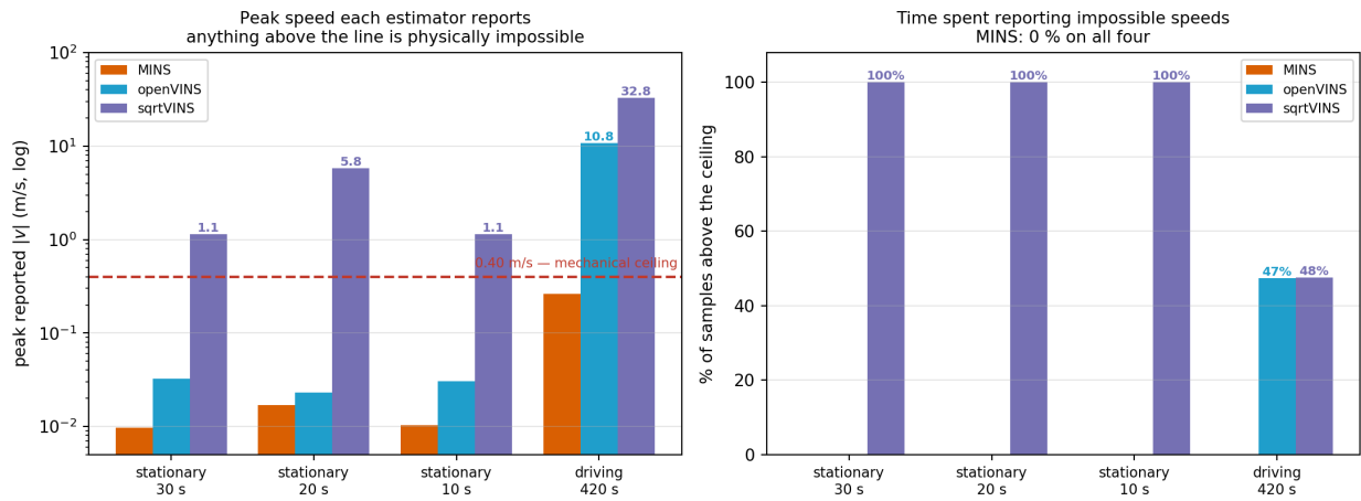
Figure 11.4: The three estimators against a constraint none of them can argue with. Left: peak reported speed, logarithmic; the dashed line is the rover’s 0.4 m/s mechanical ceiling and everything above it is impossible by construction. Right: the fraction of samples above that ceiling. MINS does not appear in the right panel because its bar is zero on all four recordings.
