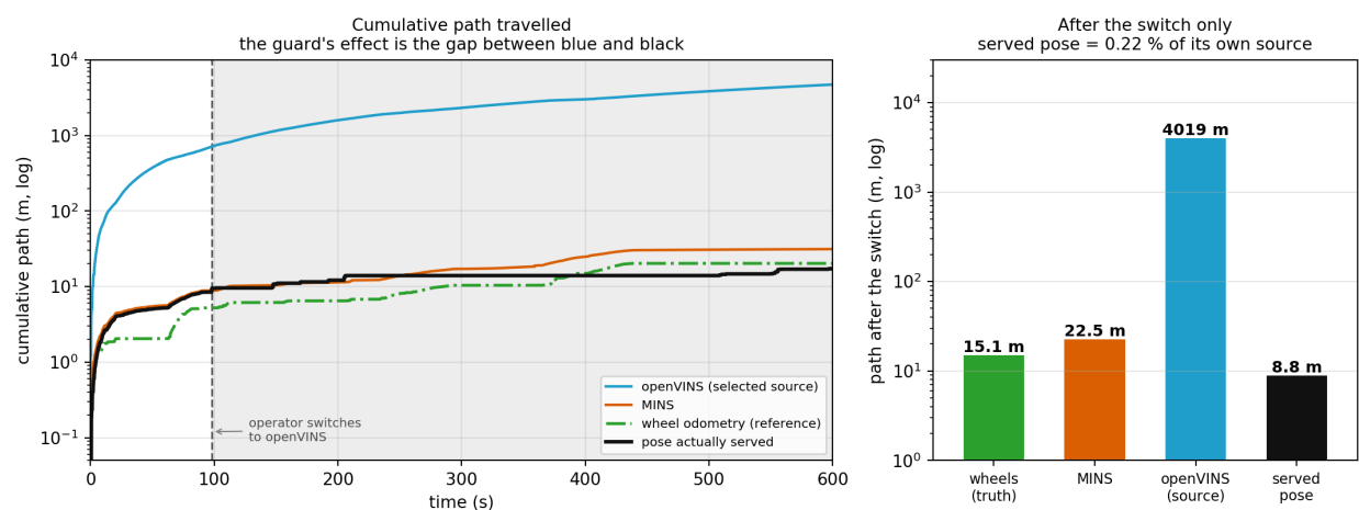
Figure 11.3: The guard under adversarial conditions, on a 600-second recording. Left: cumulative path travelled by each series, logarithmic. The dashed line marks the instant the operator selects openVINS as the served source; the shaded region is the interval during which a diverging estimator is the selected one. The blue curve is what was asked for, the black curve is what was served, and the vertical gap between them is the guard's entire contribution. Right: path accumulated after the switch only. The served pose travels 8.8 m while the source it nominally follows travels 4019 m — a suppression to 0.22 %. Wheel odometry, independent of both estimators, gives 15.1 m as the reference.
