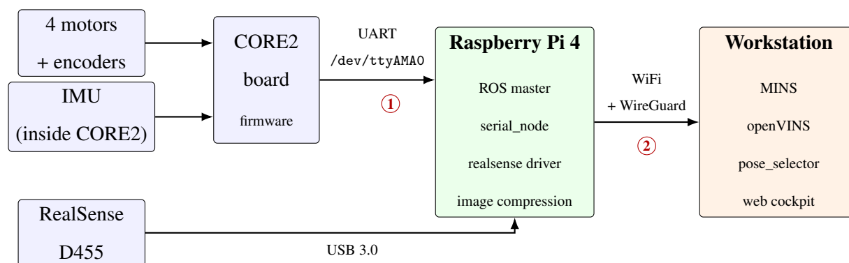
Figure D.1: The physical chain. Weak link ① : the CORE2 board talks to the Pi over a GPIO serial port ( /dev/ttyAMA0 ), not USB, a detail that misleads everyone, because unplugging USB cables cannot fix it. That link has no retransmission: if the Pi is too busy to empty the serial buffer in time, bytes are lost outright (§D.15.7). Weak link ② : the WiFi hop adds latency and jitter. Measured on this install: 0% packet loss but round-trip times of 3 to 66 ms. ROS tolerates this because everything is timestamped at the source; the video preview does not, which is why the cockpit shows a high latency badge that is honest about the video and irrelevant to the trajectories.
