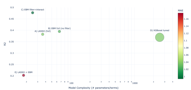
Complexity vs R2 (bubble size = training time, color = MAE)
