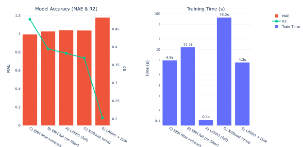
Section 14: Model Comparison Benchmark
