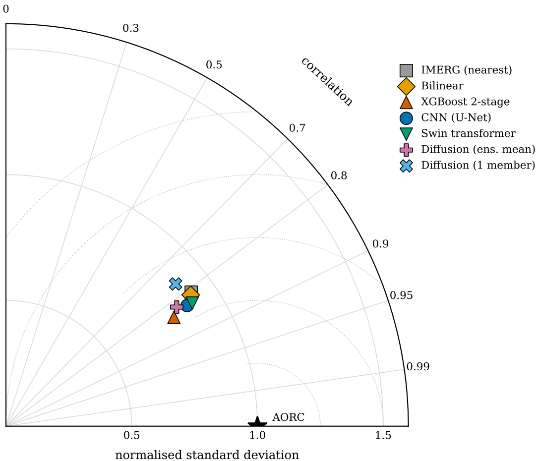
Taylor diagram, 1 km test period
