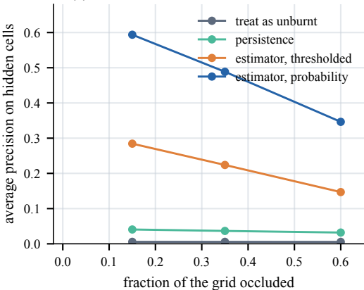
(a) does the belief match what was hidden?
