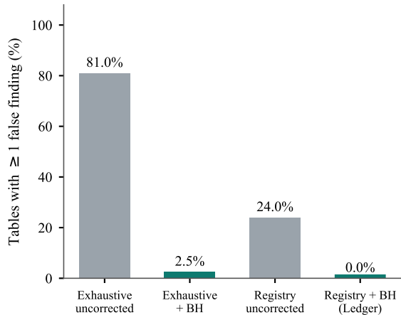
(b) Fraction of null tables contaminated
