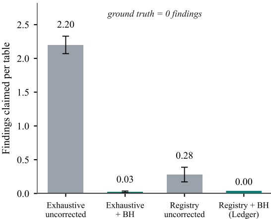
(a) Mean findings on null tables
