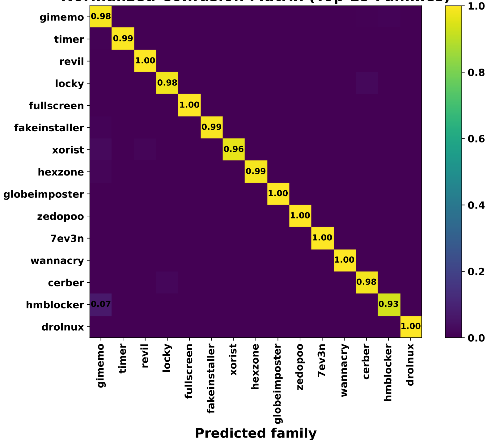
Normalized Confusion Matrix (Top 15 Families)
