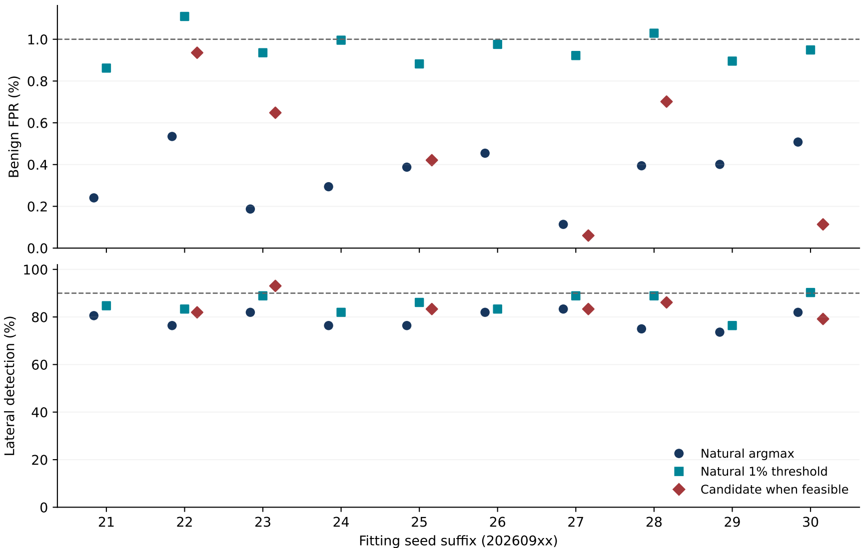
Primary verification: all ten fitting seeds
