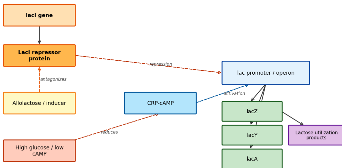
Figure B. Regulatory wiring emphasis. Orange = lacI gene to protein (RegulonDB first-class entities). No AND-gate diamonds; combinatorial logic is left to the reader.
