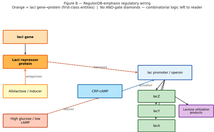
Figure B. Regulatory wiring emphasis. Orange = lacI gene to protein (RegulonDB first-class entities). No AND-gate diamonds; combinatorial logic is left to the reader.
