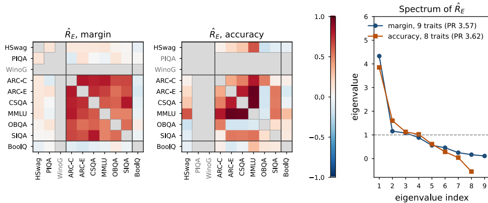
Figure 3. Cross-half correlation estimates across the 125 configurations, margins on the left and accuracy in the center, with undefined variances shown in grey and eigenvalue spectra on the right. The accuracy estimate has a negative eigenvalue, and its spectrum is a diagnostic of the moment estimate rather than a valid population correlation spectrum. PR is the spectral participation ratio, 3.57 on the nine margin traits and 3.62 on the eight accuracy traits after clipping that eigenvalue.
