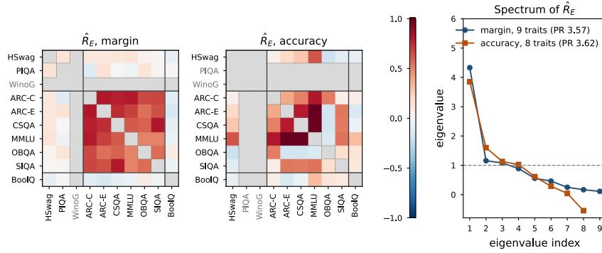
Figure 2. Cross-half correlation estimates across the 125 configurations, margins on the left and accuracy in the center, with undefined variances shown in grey and eigenvalue spectra on the right. The accuracy estimate has a negative eigenvalue, and its spectrum is a diagnostic of the moment estimate rather than a valid population correlation spectrum. PR is the spectral participation ratio, 3.57 on the nine margin traits and 3.62 on the eight accuracy traits after clipping that eigenvalue.
