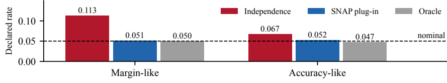
Figure 1. Share of 4,000 simulated null comparisons that declare a difference at a nominal 0.05 level. Scaling the independence error bar by the SNAP estimate returns the margin rate to the oracle’s.
