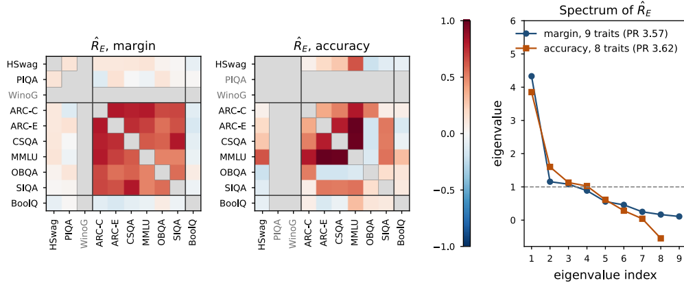
Figure 1. Cross-half correlation estimates across the 125 configurations, with undefined variances shown in grey. The accuracy estimate has a negative eigenvalue, so its spectrum is a diagnostic of the moment estimate rather than a valid population correlation spectrum.
