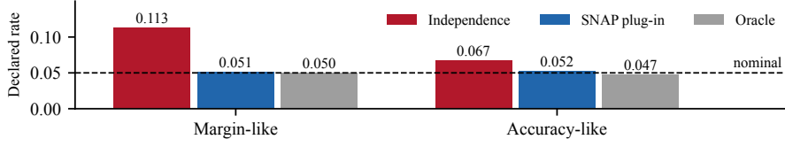
Figure 1. Share of 4,000 simulated null comparisons that declare a difference at a nominal 0.05 level. Scaling the independence error bar by the SNAP estimate from the same population returns the margin rate to the oracle’s.
