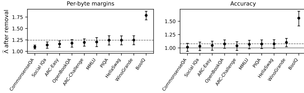
Figure 1. Inflation after removing each benchmark in turn, with nominal 95% recipe-cluster intervals. The solid line marks one and the dashed line the full ten-benchmark estimate. On margins every removal leaves an interval that excludes one, and the estimate runs from 1.096 without CommonsenseQA to 1.786 without BoolQ.
