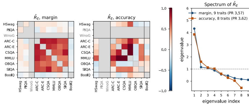
Figure 2. Cross-half correlation estimates across the 125 configurations, margins on the left and accuracy in the center, with undefined variances shown in grey and eigenvalue spectra on the right. The accuracy estimate has a negative eigenvalue, and its spectrum is a diagnostic of the moment estimate rather than a valid population correlation spectrum. PR is the spectral participation ratio, 3.57 on the nine margin traits and 3.62 on the eight accuracy traits after clipping that eigenvalue.
