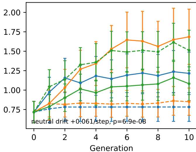
Qualifier retention
