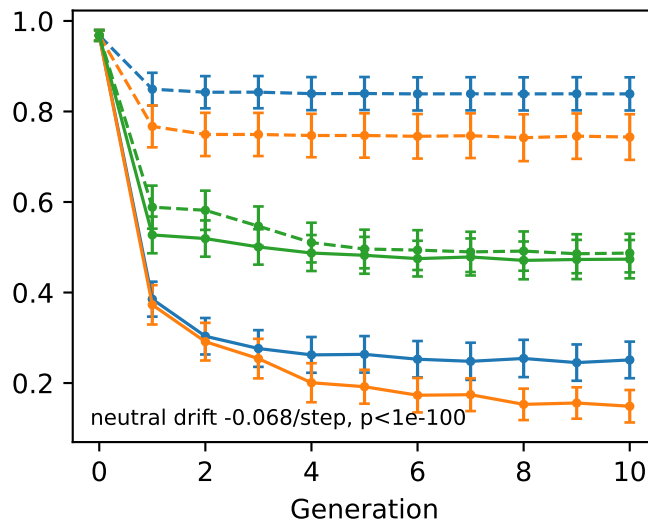
Bidirectional entailment
