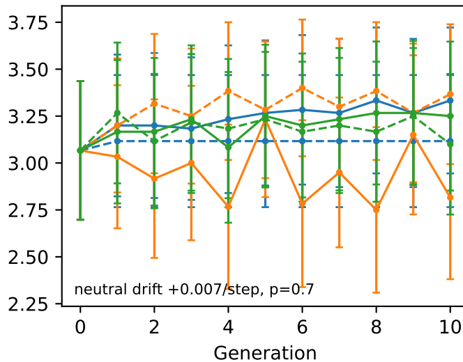
Bidirectional entailment
