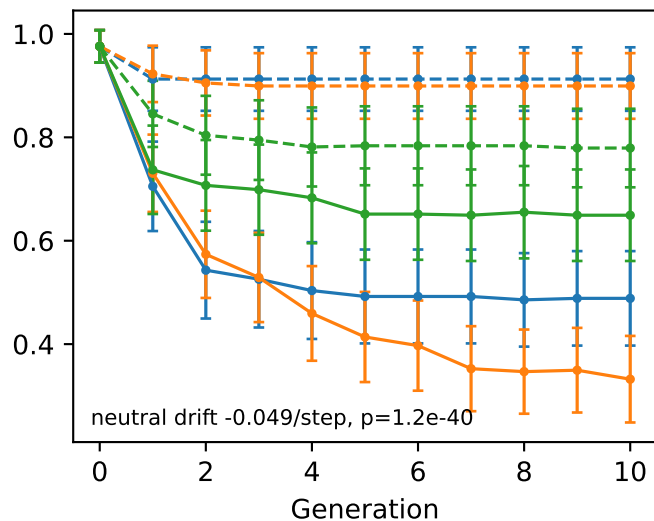
Qualifier retention
