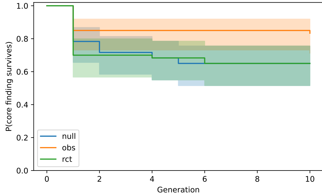
conservative regime
