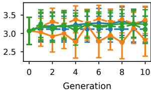
Bidirectional entailment
