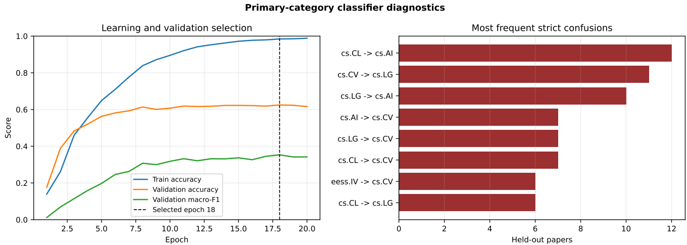
Figure 1: Left: training accuracy continued toward 1.0 while validation accuracy and macro-F1 flattened; the dashed line marks the selected epoch. Right: strict primary-label errors concentrate among overlapping computing categories. Counts come from the 1,157-paper test set.
