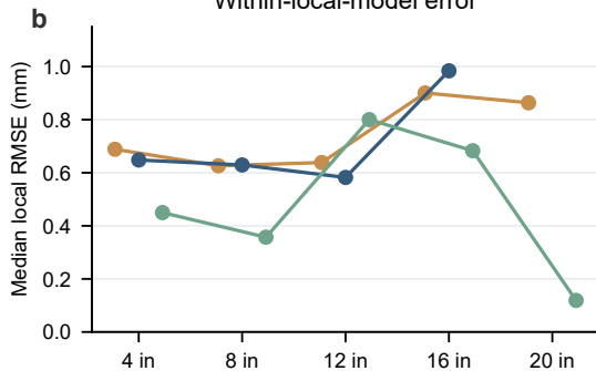
Within-local-model error
