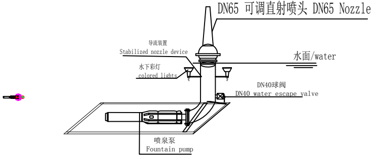
喷泉剖面图 Fountain profile drawing
