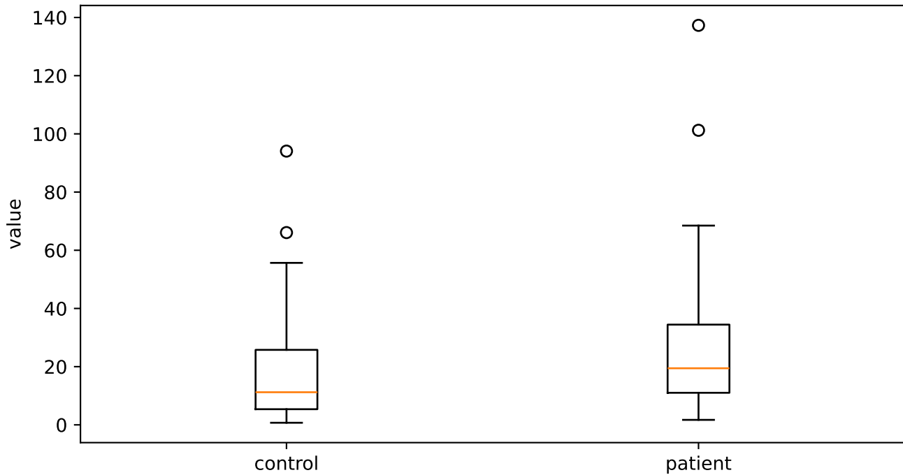
std_f0_hertz
