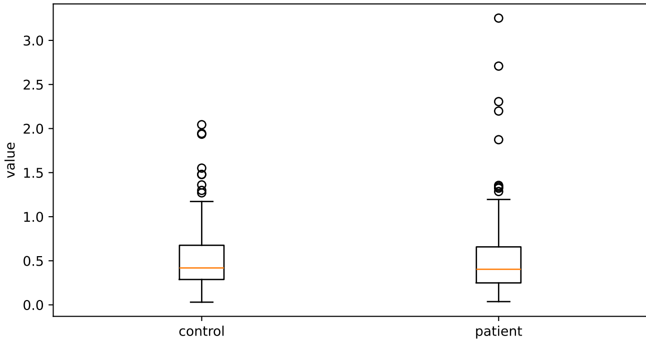
loudness_sma3_amean
