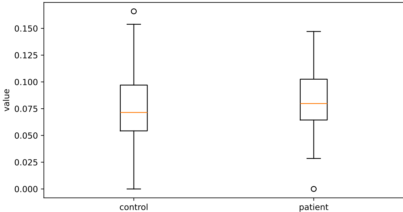
F3frequency_sma3nz_stddevNorm
