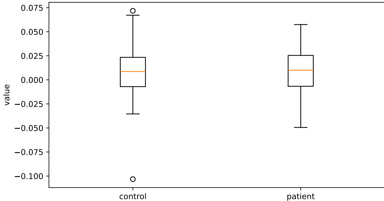
slopeV0-500_sma3nz_amean
