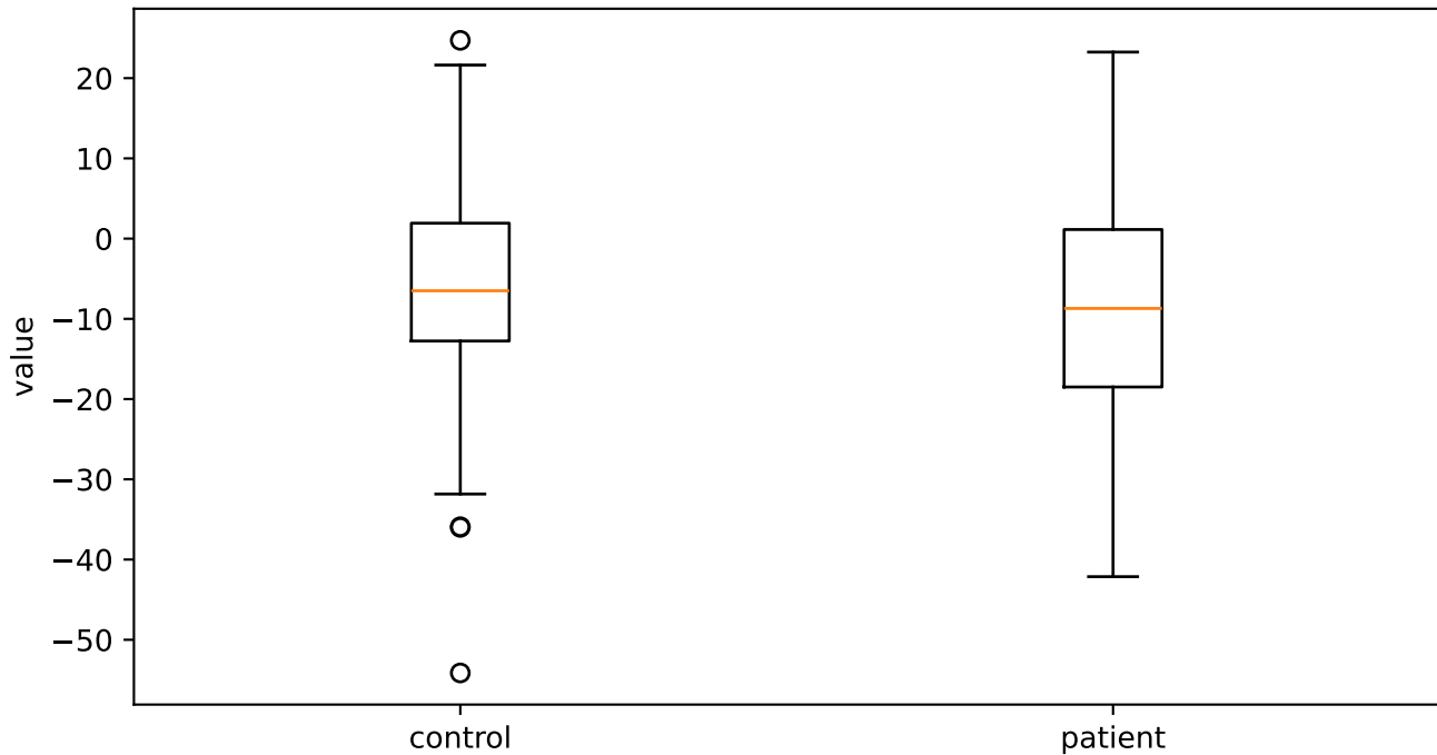
mfcc4V_sma3nz_amean
