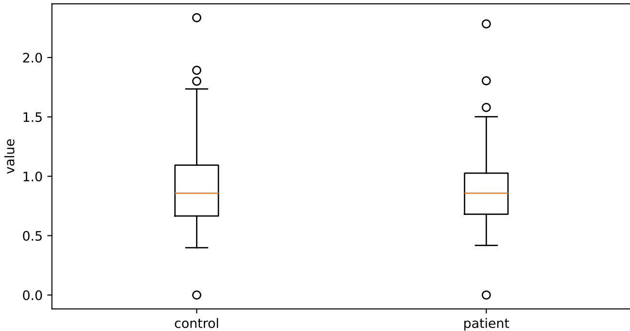
shimmerLocaldB_sma3nz_stddevNorm
