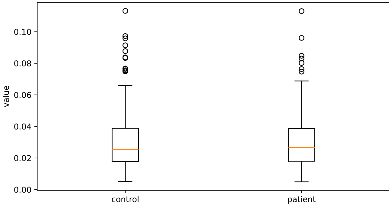
apq3_shimmer
