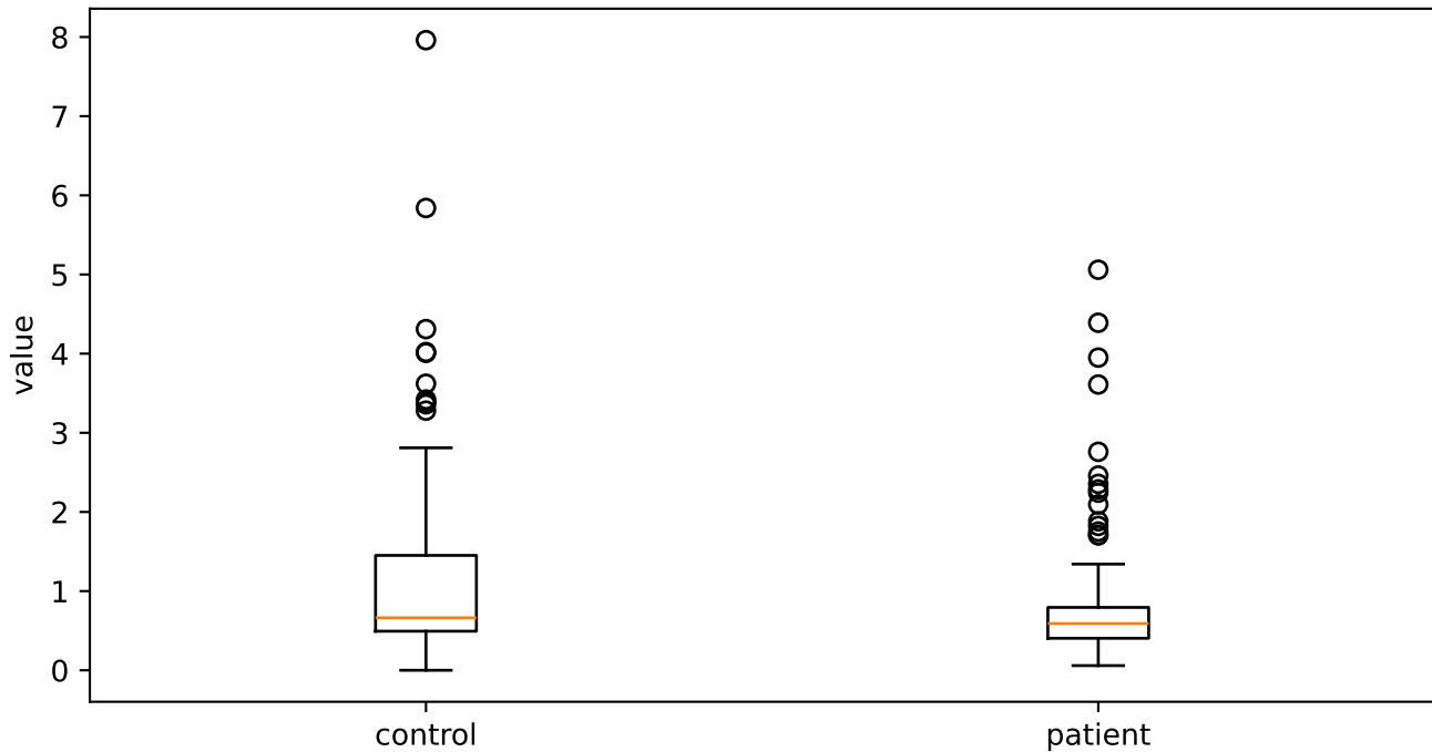
MeanUnvoicedSegmentLength
