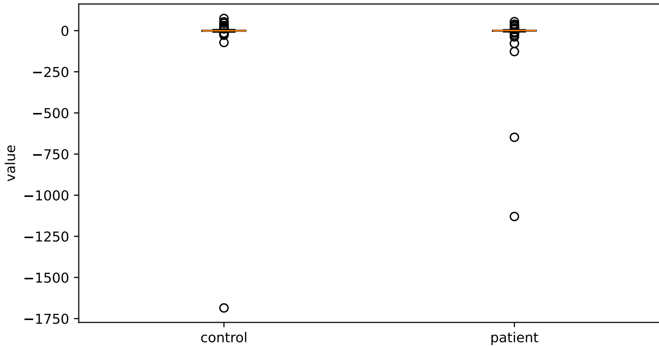
mfcc3_sma3_stddevNorm
