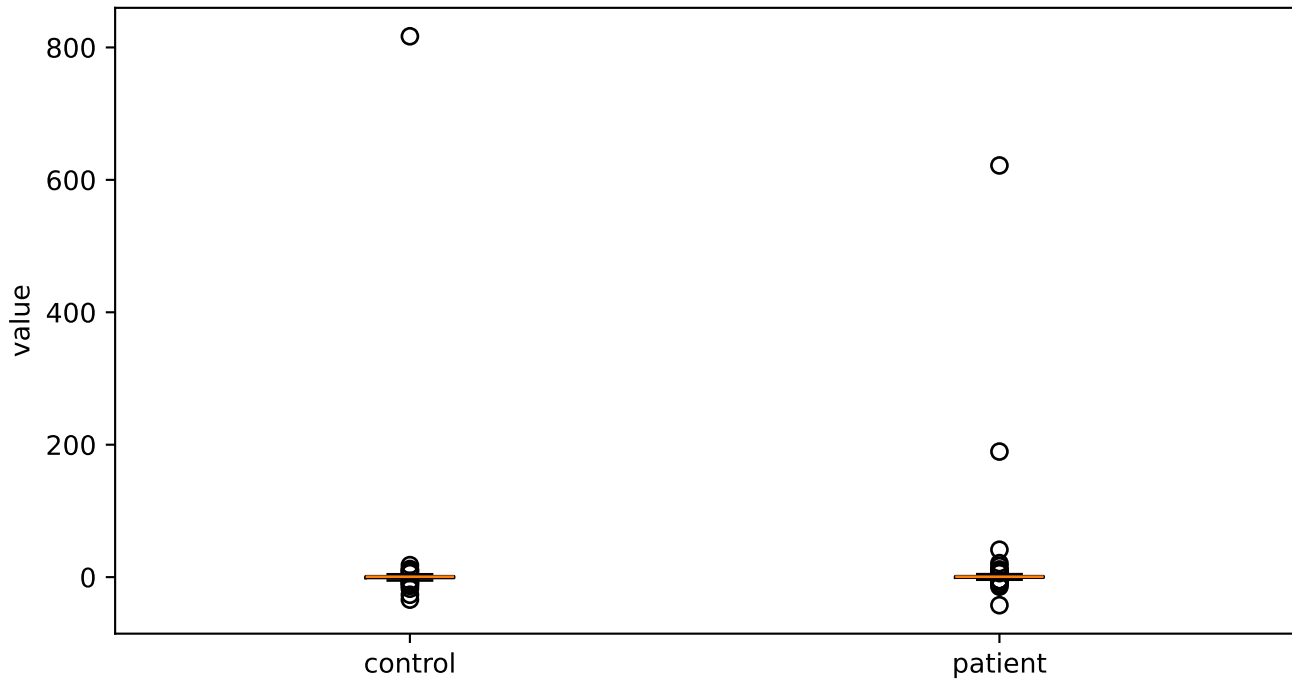
mfcc2_sma3_stddevNorm
