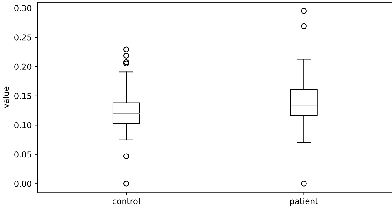
F1bandwidth_sma3nz_stddevNorm
