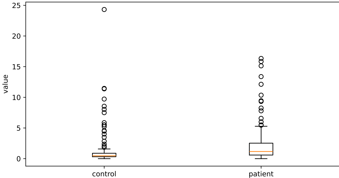
F0semitoneFrom27.5Hz_sma3nz_pctlrange0-2
