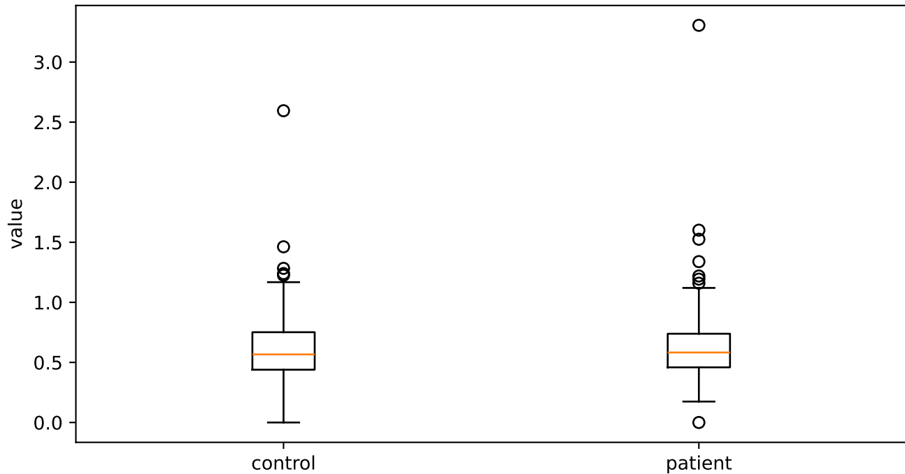
spectralFluxV_sma3nz_stddevNorm
