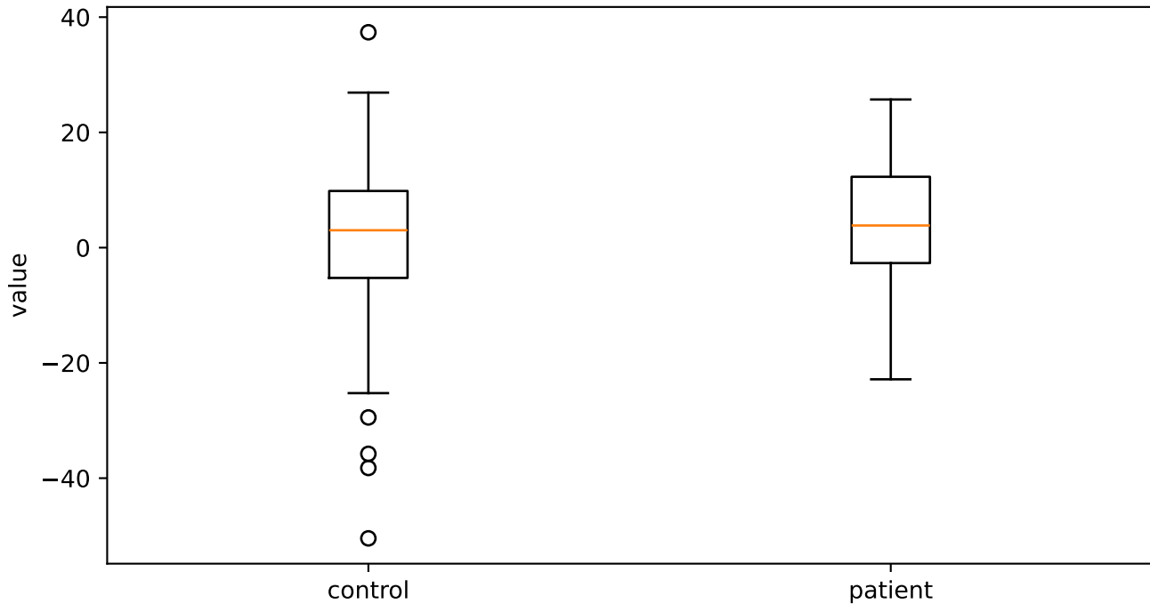
mfcc2V_sma3nz_amean
