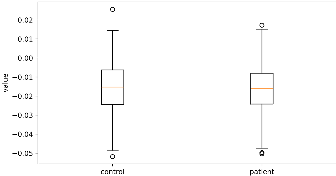
slopeV500-1500_sma3nz_amean
