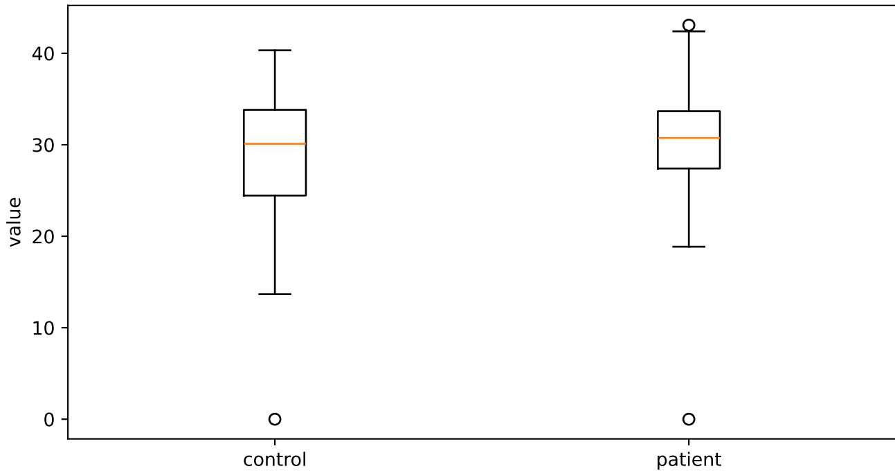
F0semitoneFrom27.5Hz_sma3nz_percentile80.0
