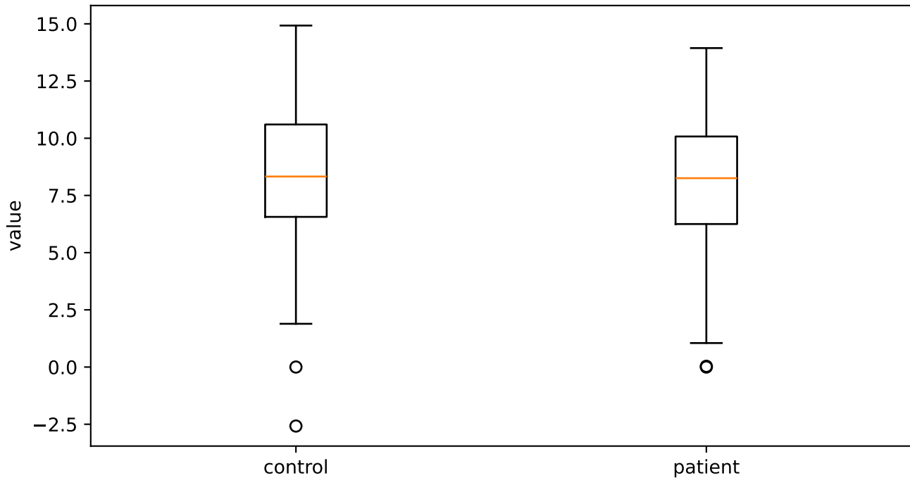
HNRdBACF_sma3nz_amean
