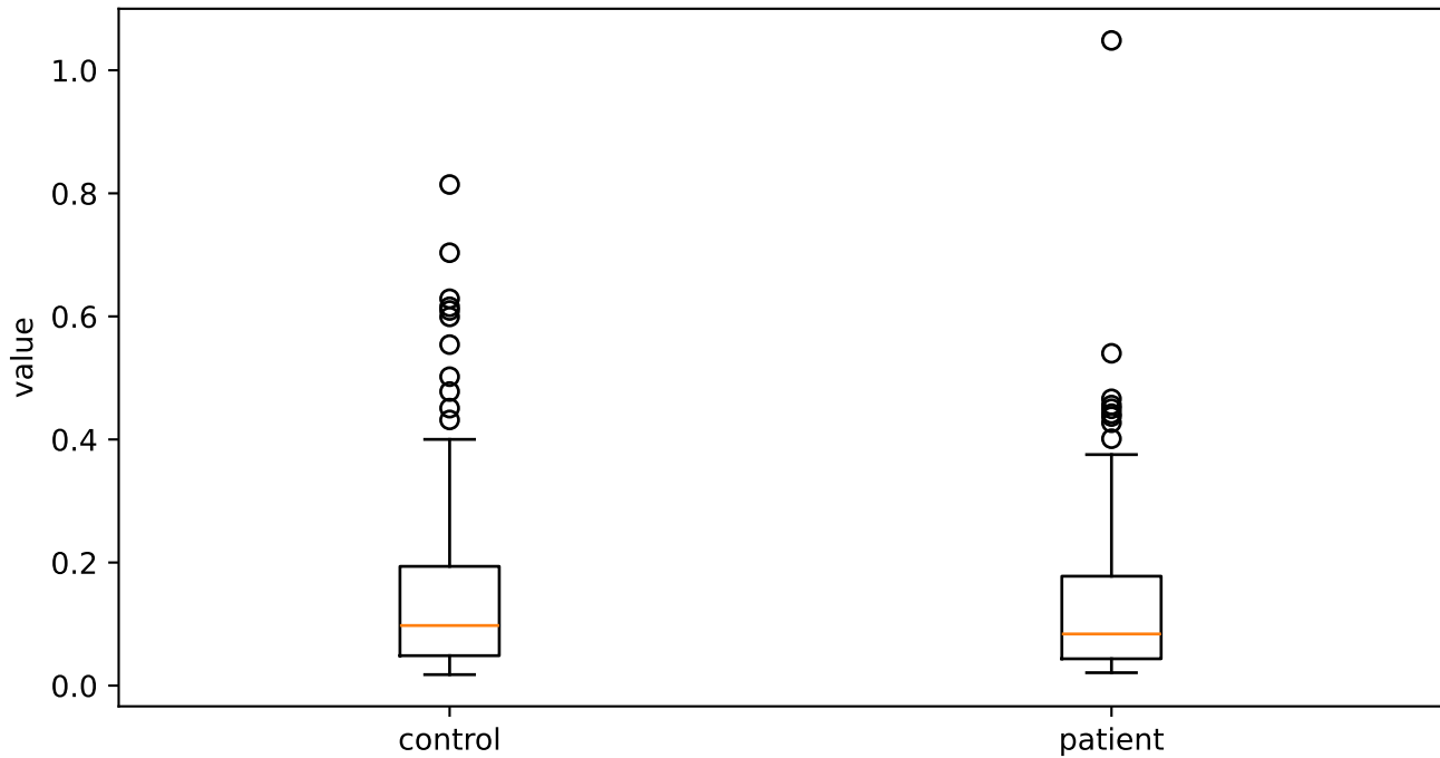
loudness_sma3_percentile20.0
