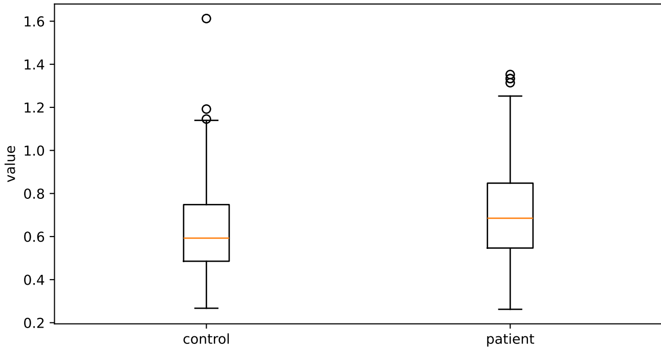
loudness_sma3_stddevNorm
