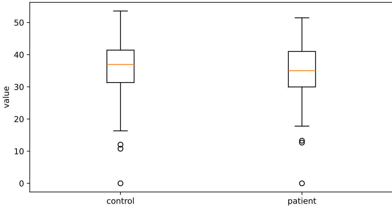
mfcc1V_sma3nz_amean
