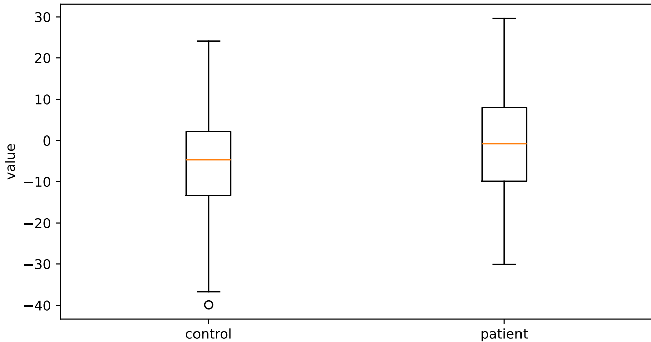
mfcc3V_sma3nz_amean
