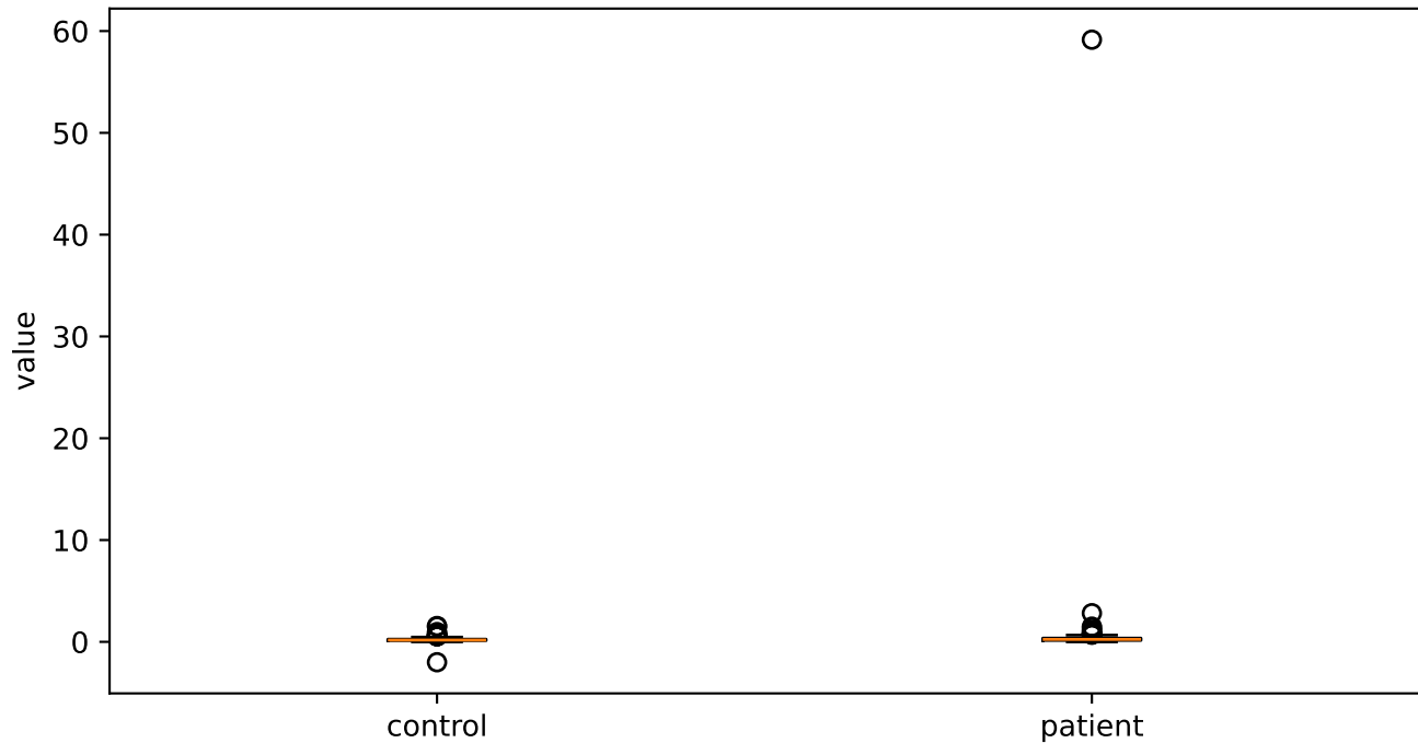
HNRdBACF_sma3nz_stddevNorm
