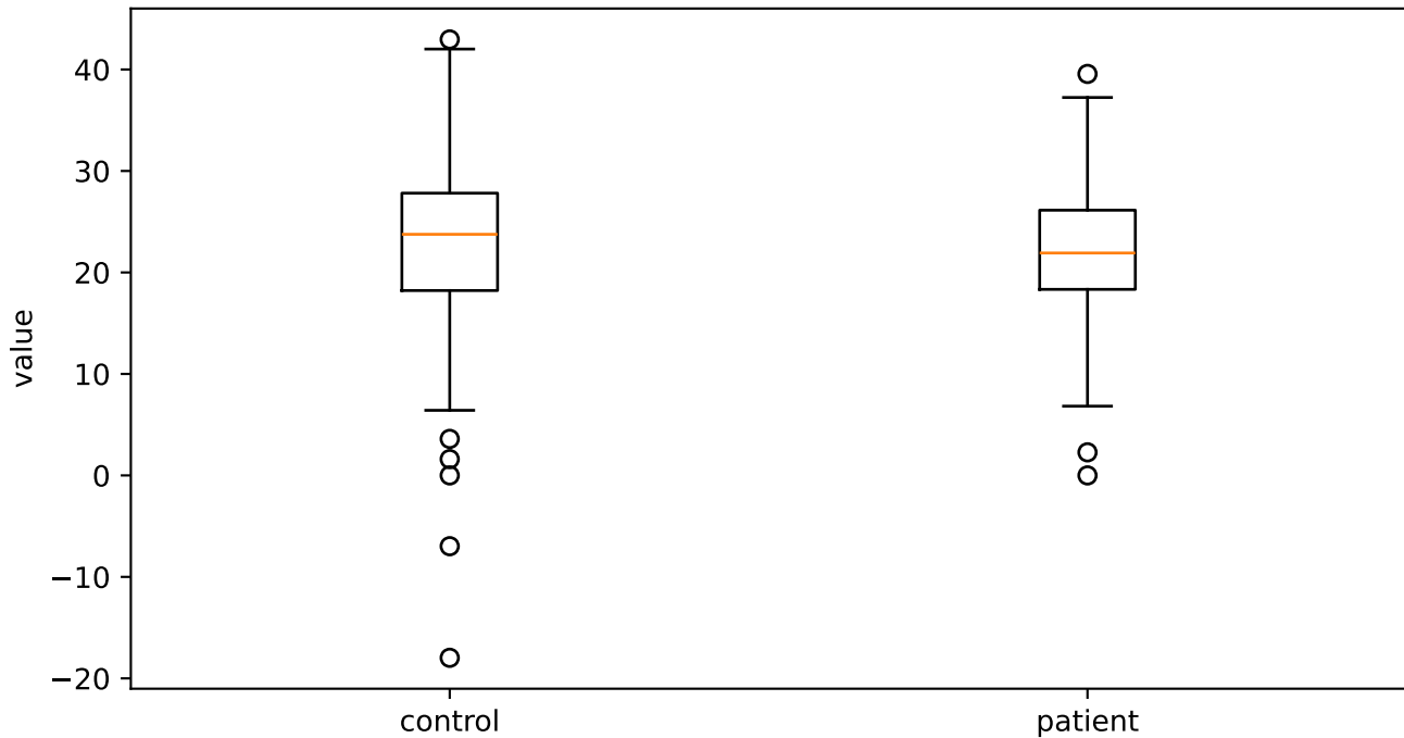
logRelF0-H1-A3_sma3nz_amean
