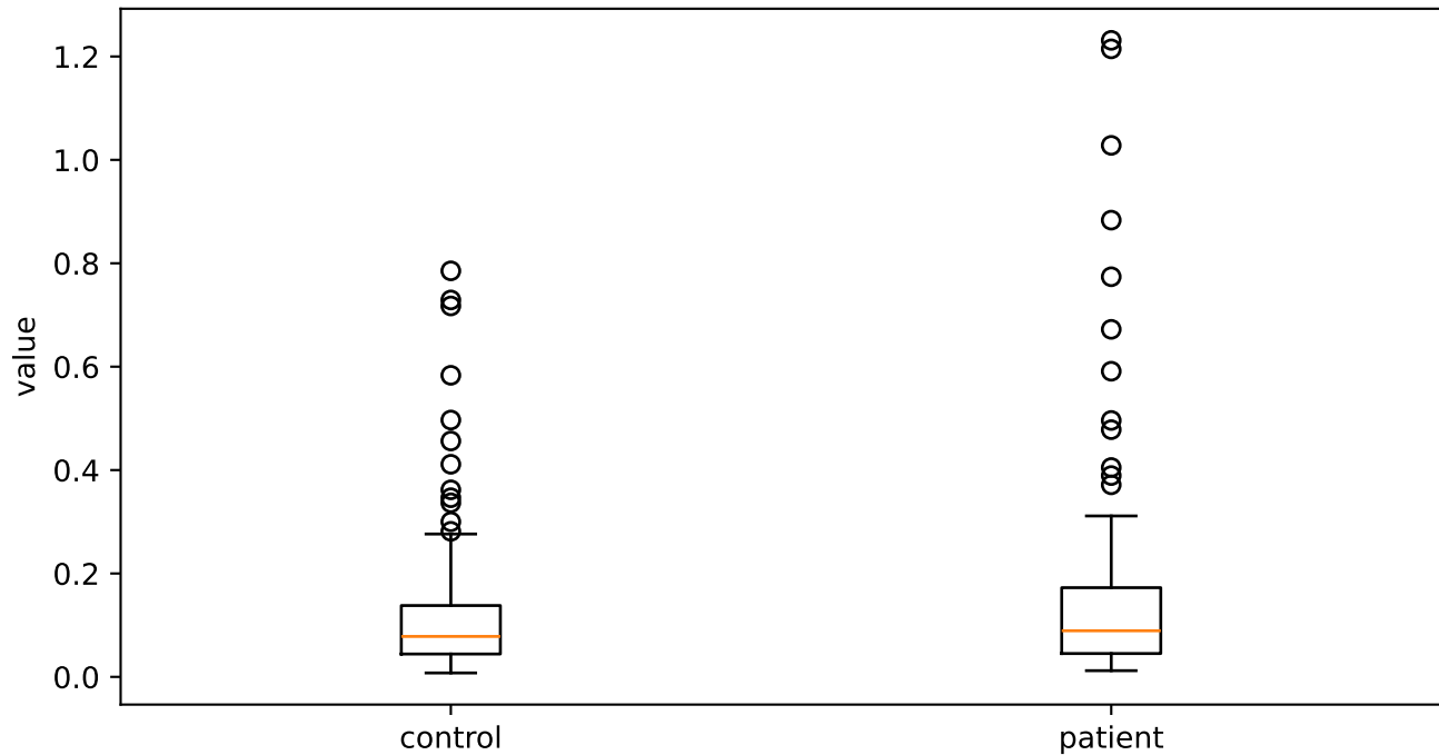
spectralFlux_sma3_amean
