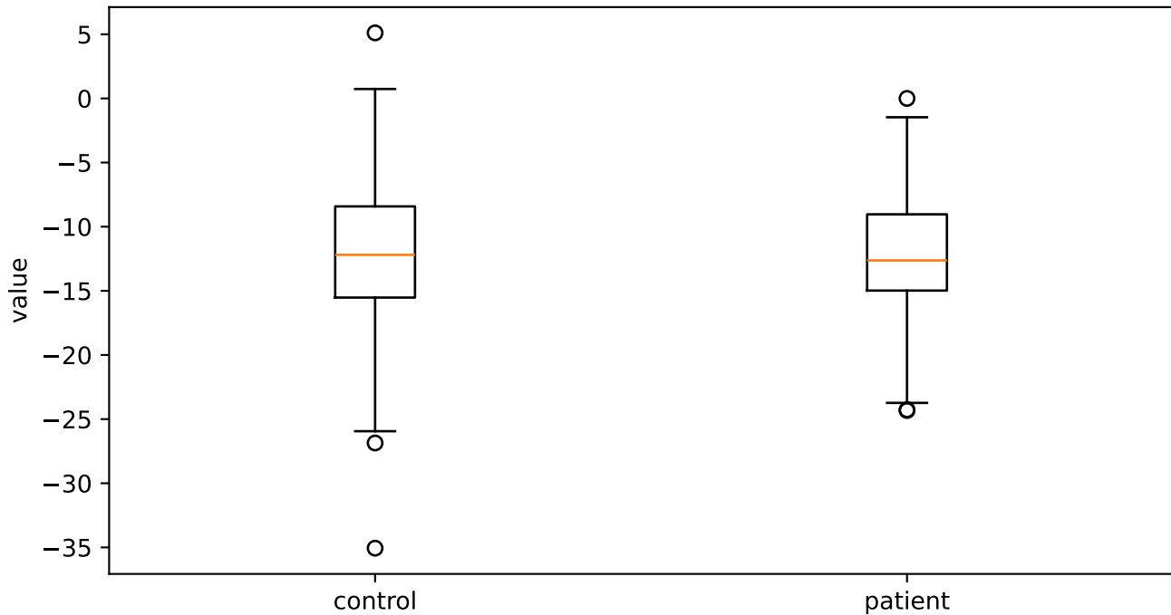
alphaRatioV_sma3nz_amean
