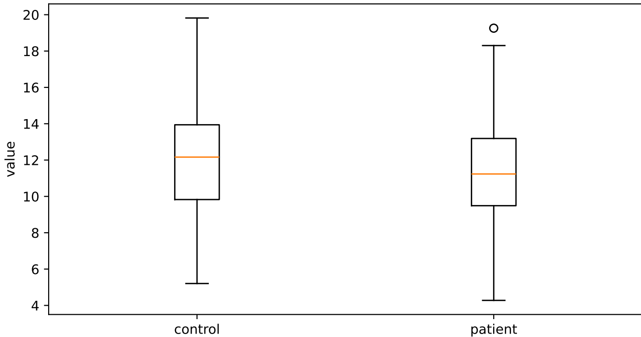
cepstral_peak_prominence_mean
