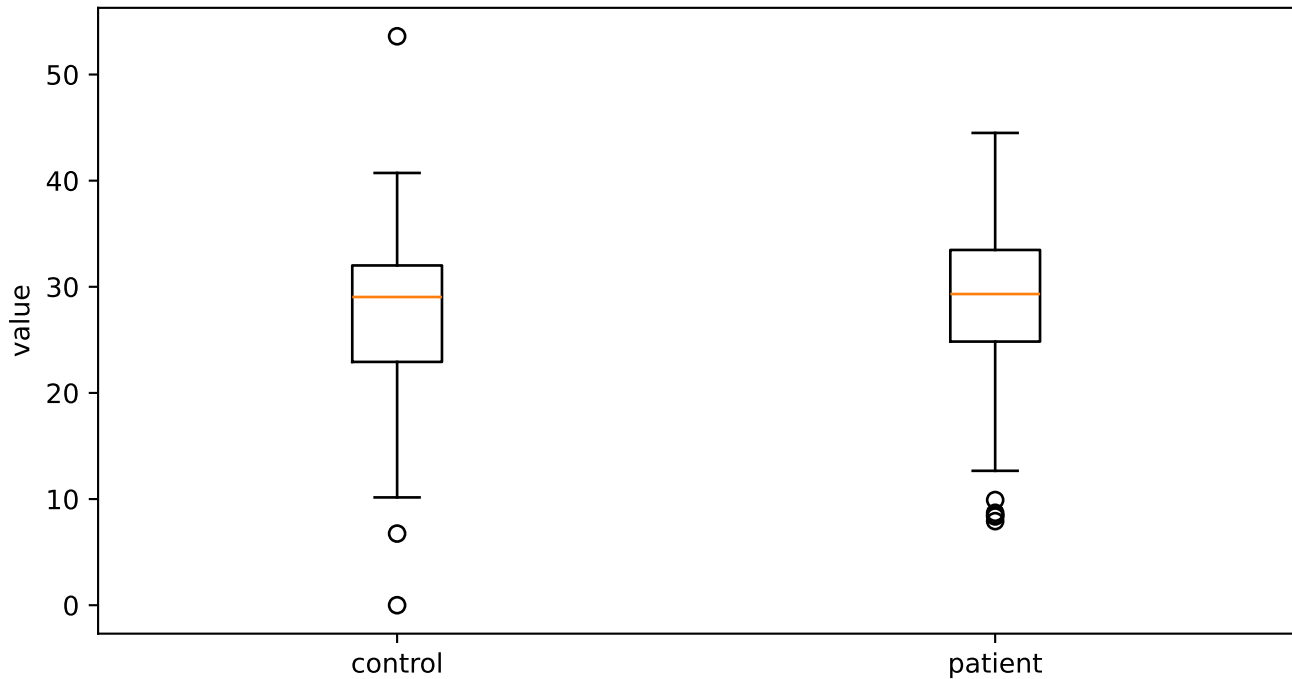
hammarbergIndexUV_sma3nz_amean
