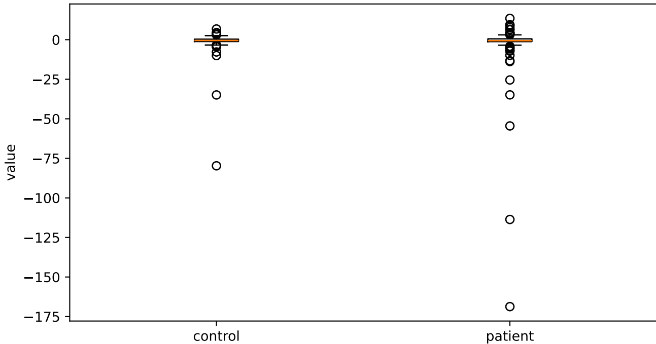
mfcc4V_sma3nz_stddevNorm
