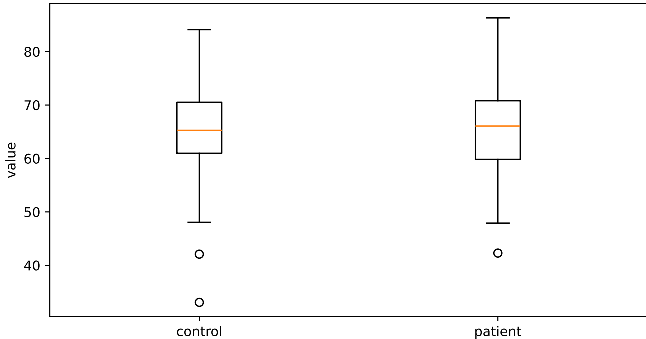
mean_intensity_db
