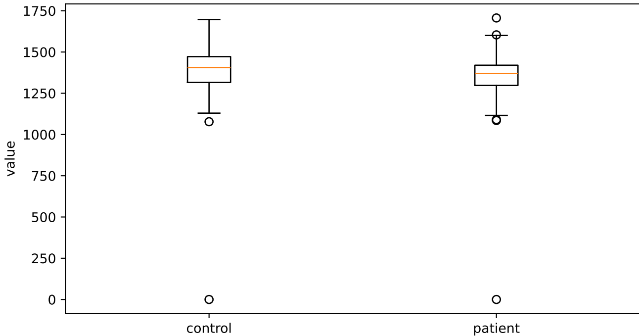
F1bandwidth_sma3nz_amean
