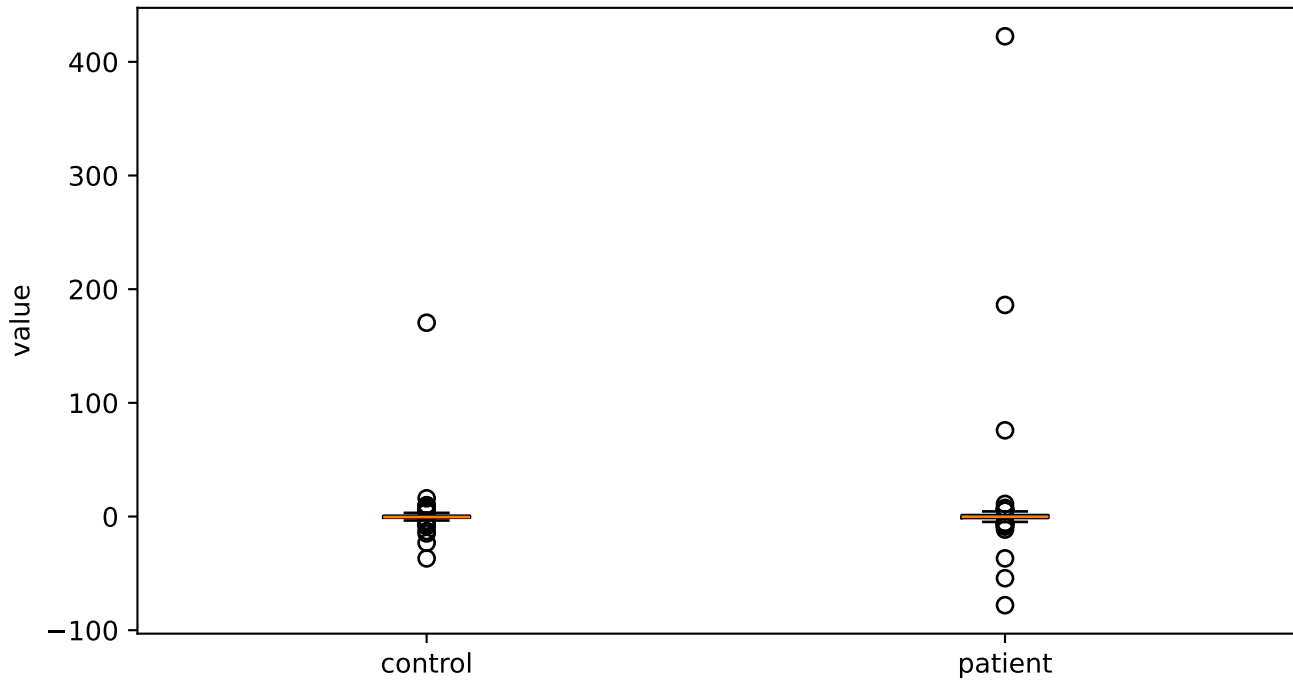
mfcc3V_sma3nz_stddevNorm
