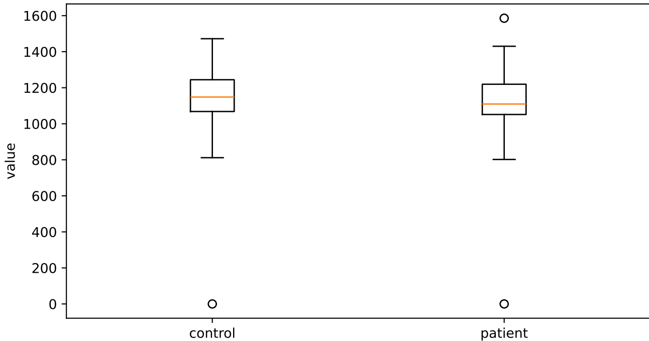
F2bandwidth_sma3nz_amean
