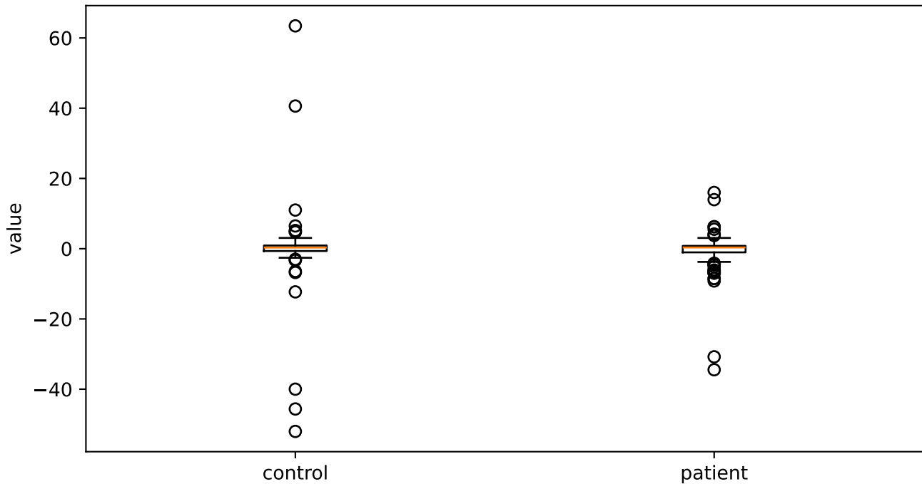
mfcc2V_sma3nz_stddevNorm
