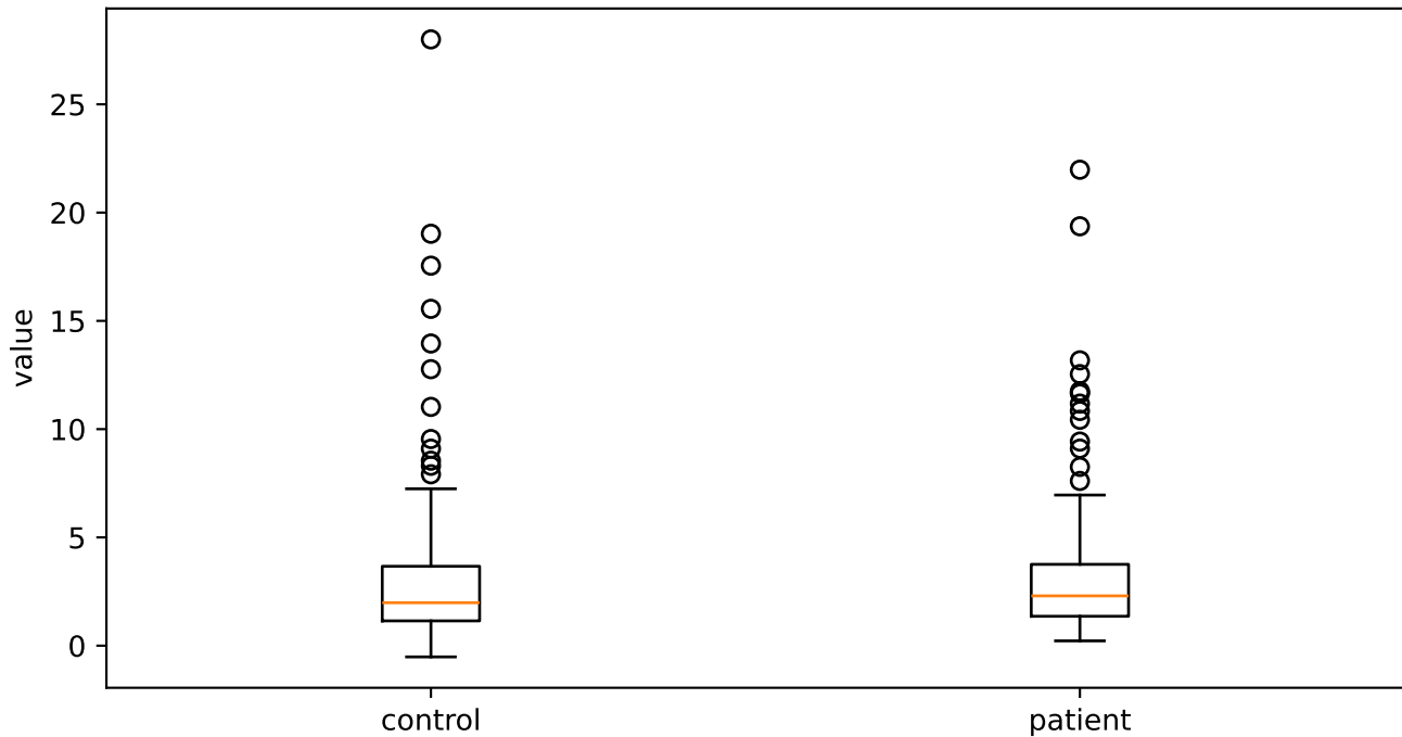
loudness_sma3_meanRisingSlope
