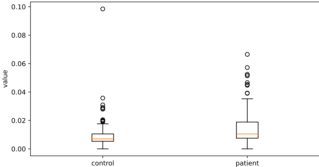
jitterLocal_sma3nz_amean
