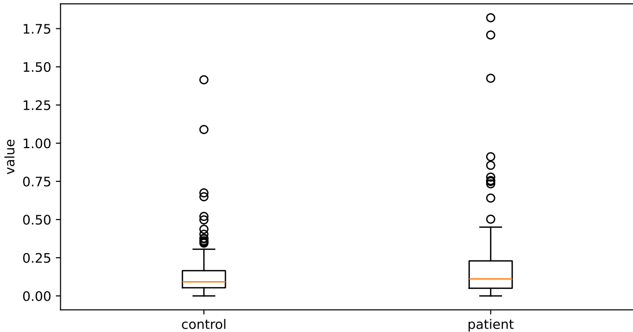
spectralFluxV_sma3nz_amean
