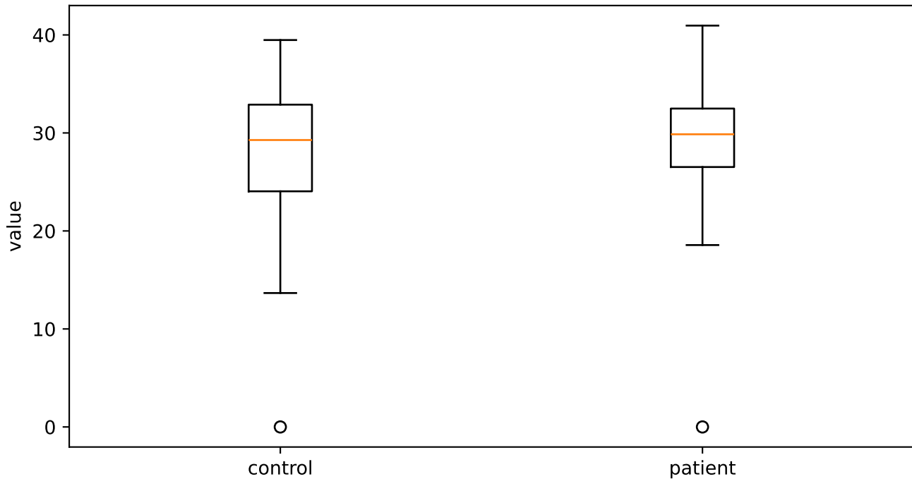
F0semitoneFrom27.5Hz_sma3nz_amean
