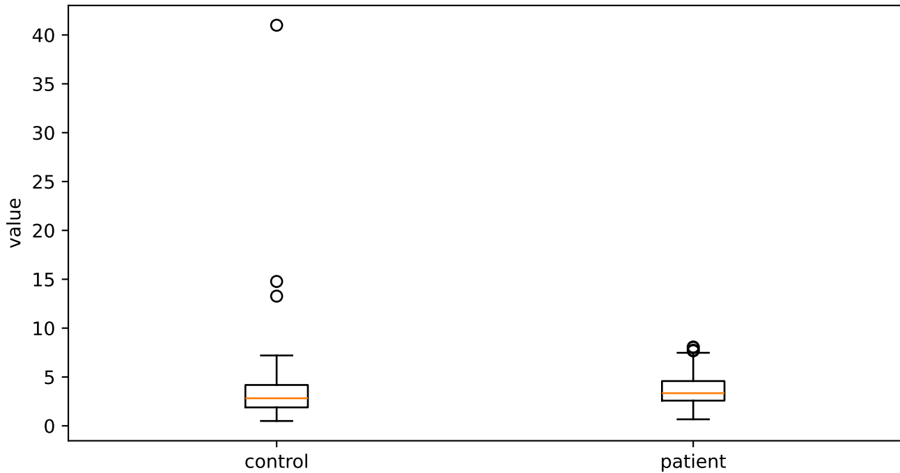
spectral_skewness
