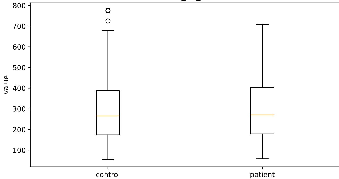
mean_b1_loc
