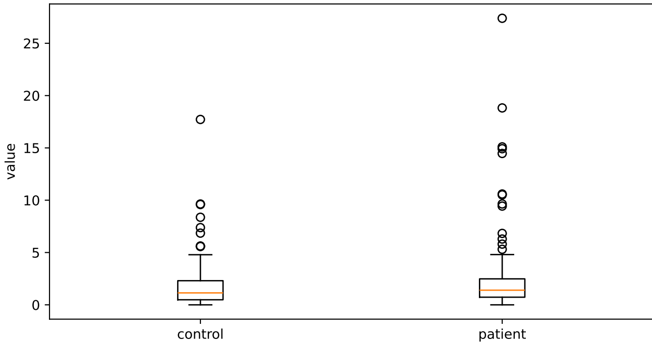
loudness_sma3_stddevFallingSlope
