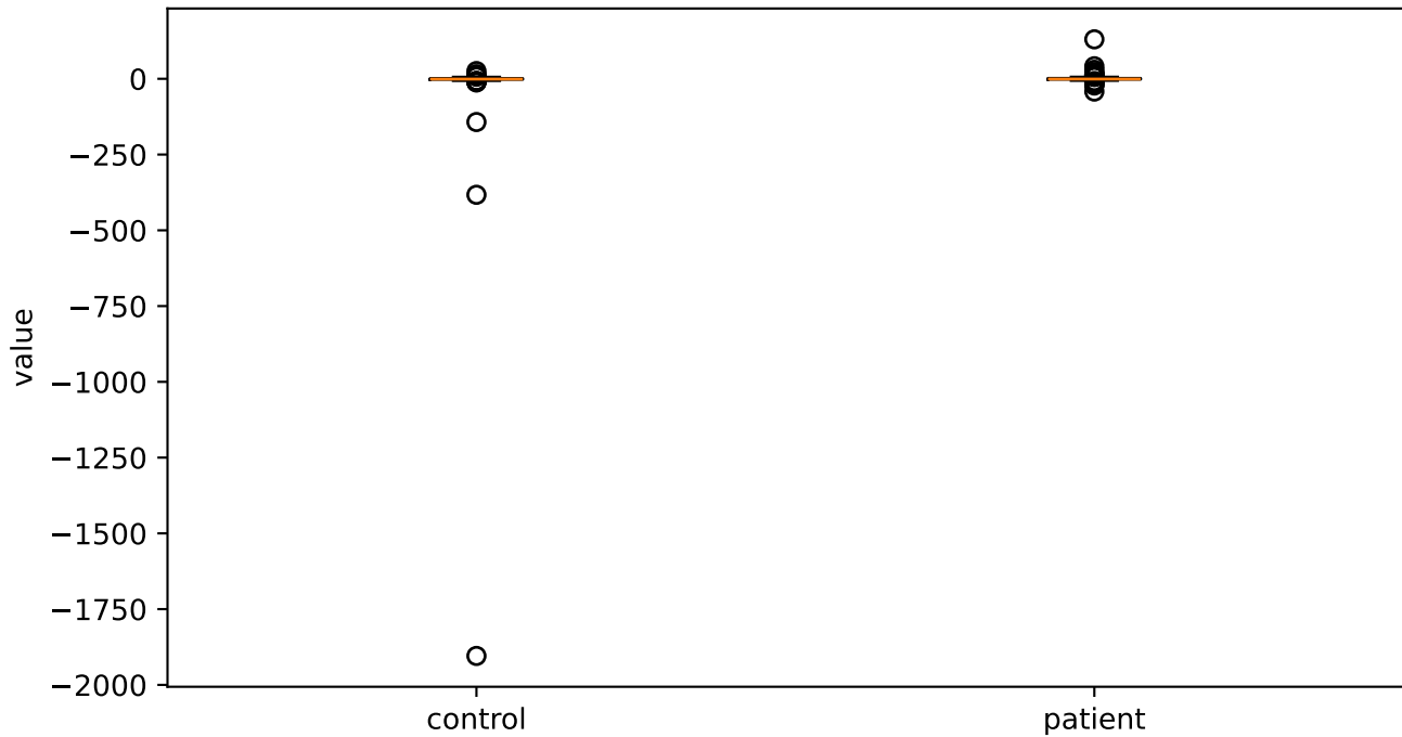
mfcc4_sma3_stddevNorm
