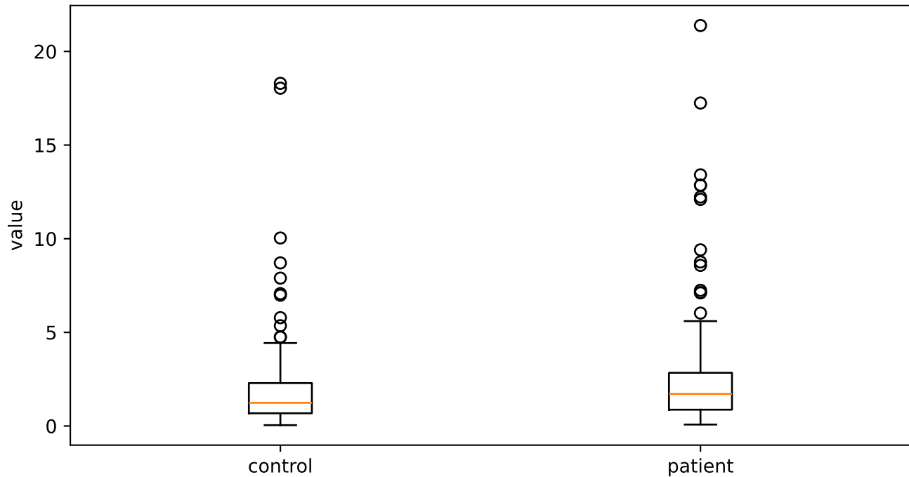
loudness_sma3_meanFallingSlope
