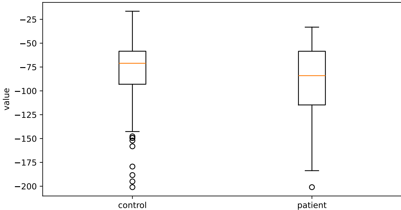
F2amplitudeLogRelF0_sma3nz_amean
