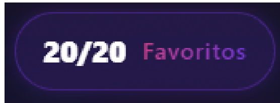
Counter at 20/20.
