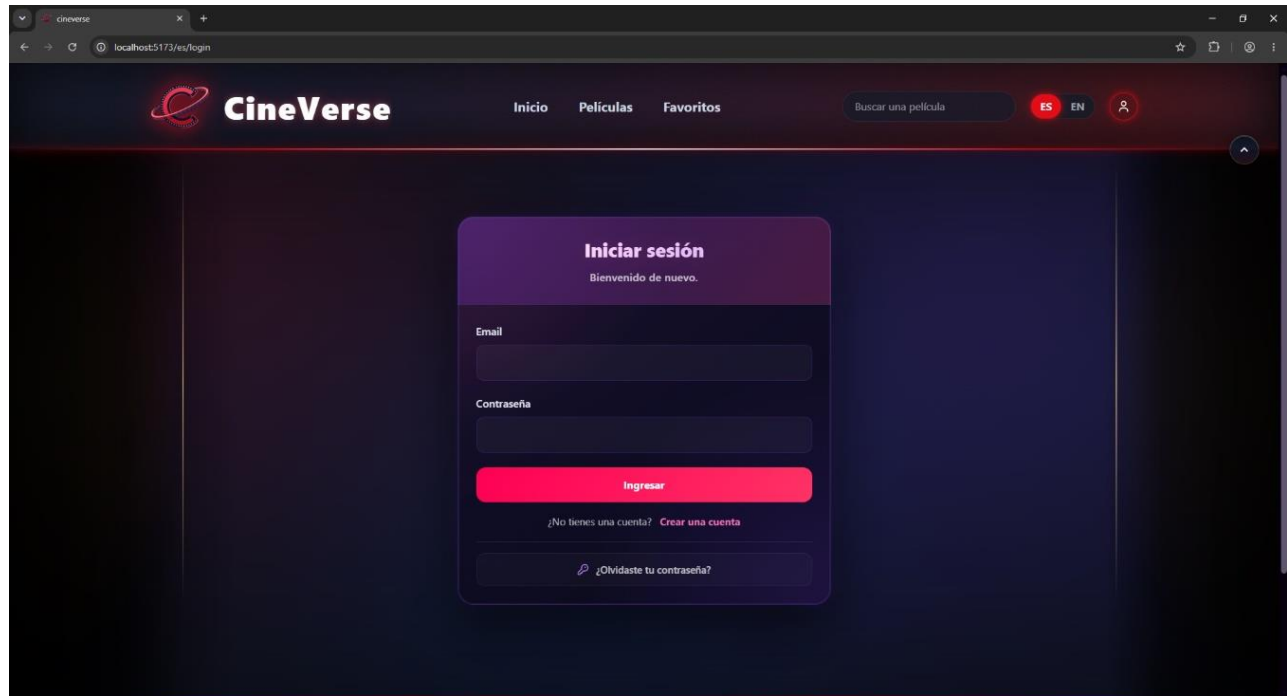
Sign-in screen.
