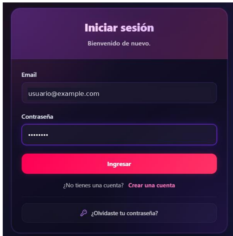
Expanded form.
