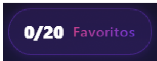
Counter at 0/20.
