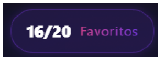
Updated counter.
