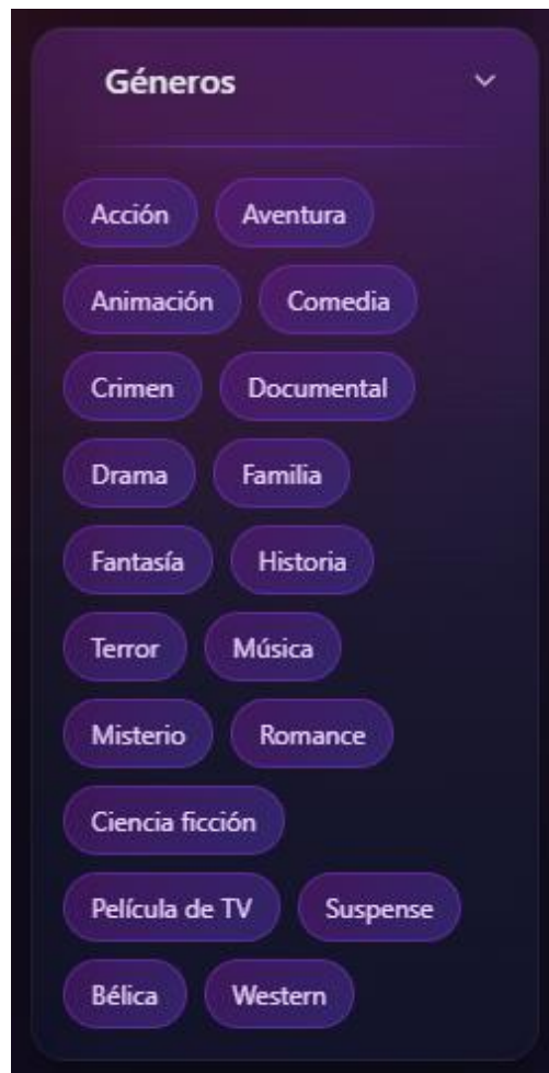
Genre selection.
