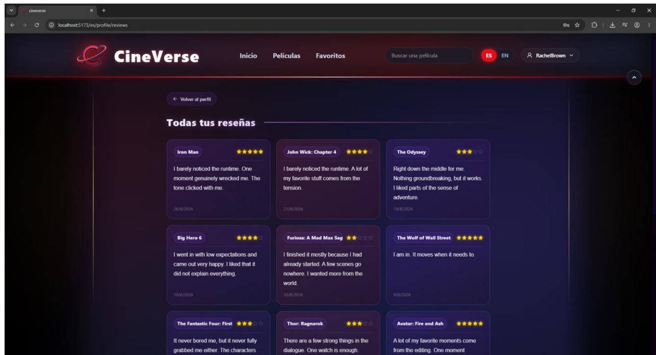
Expanded list.
