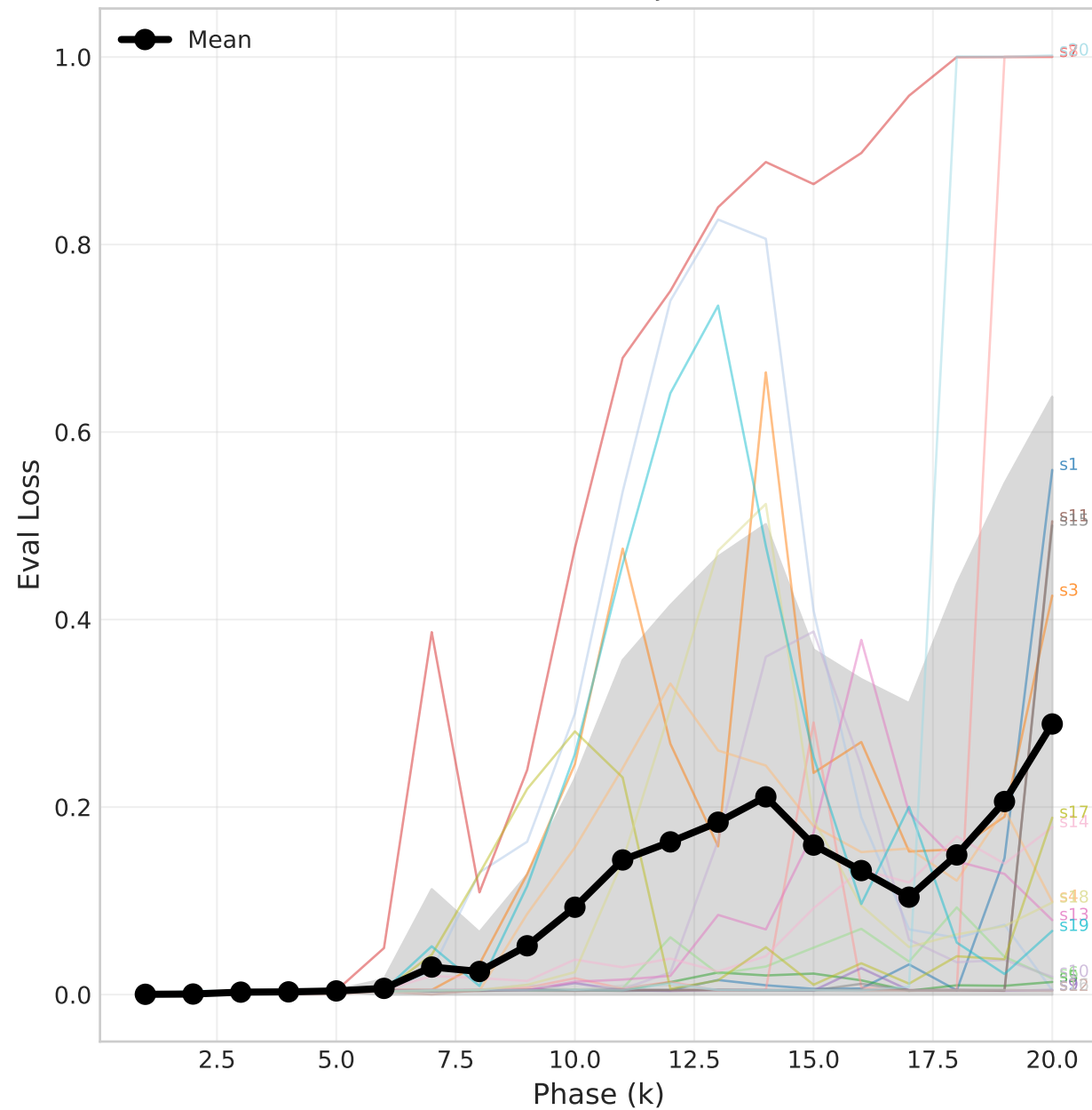
CoT: All Loss Trajectories
