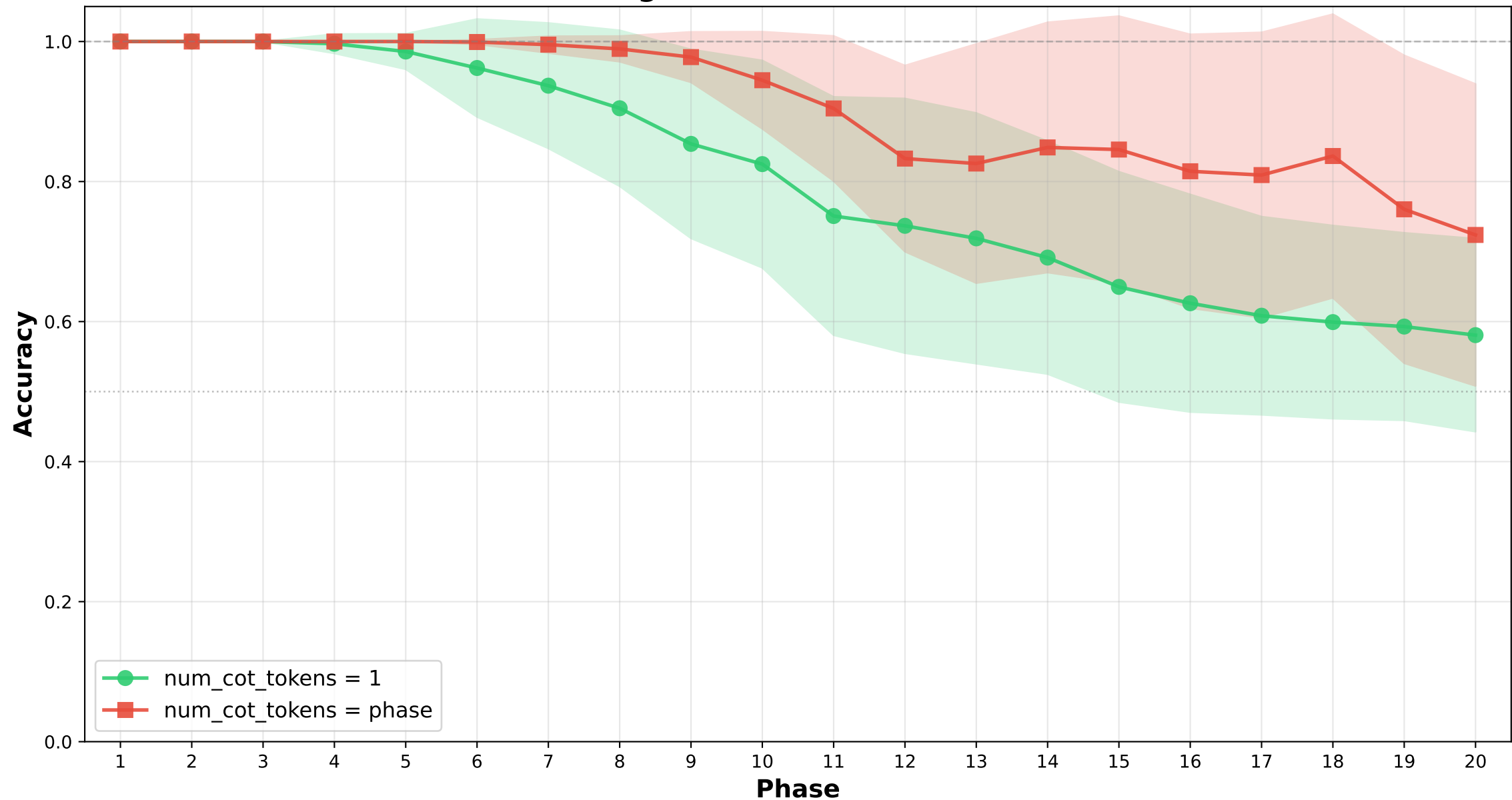
Accuracy per Phase: Comparison of CoT Token Strategies (Shaded region = \pm 1 std across 20 seeds)
