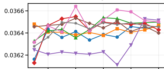
Hamming Loss
