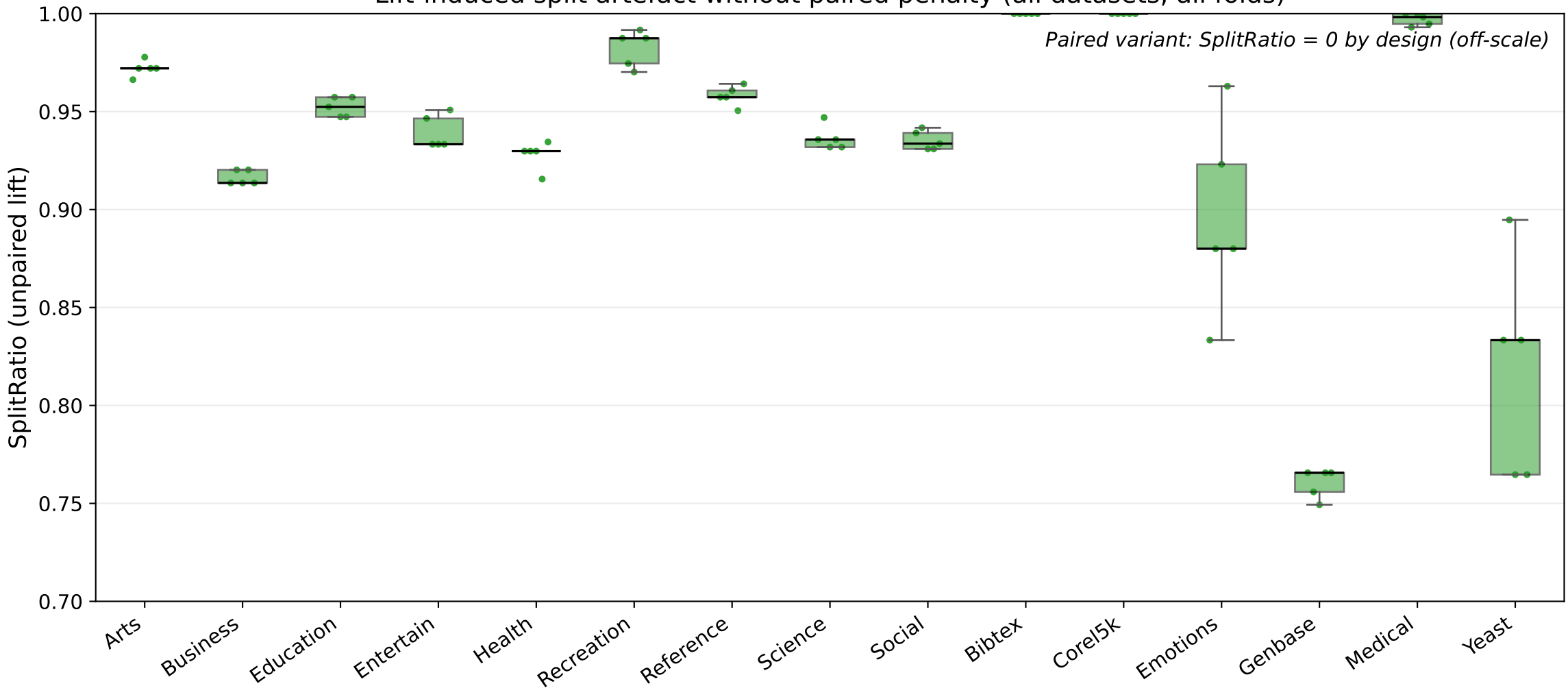
Lift-induced split artefact without paired penalty (all datasets, all folds)
