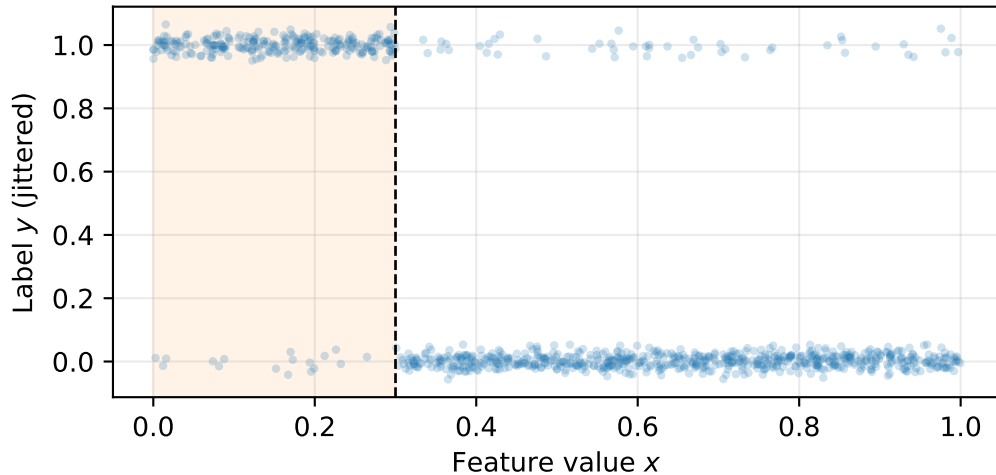
(a) Synthetic data (pos rate=0.31, flip=0.05)
