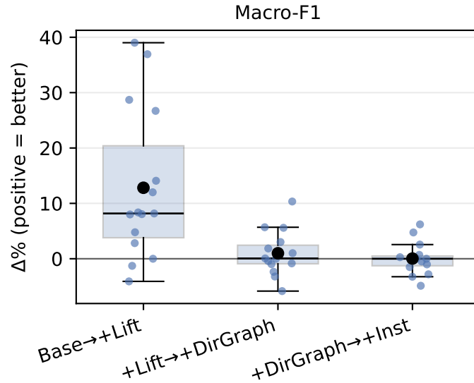
Additive ablation: per-dataset relative gains at p = 20\% selected features
