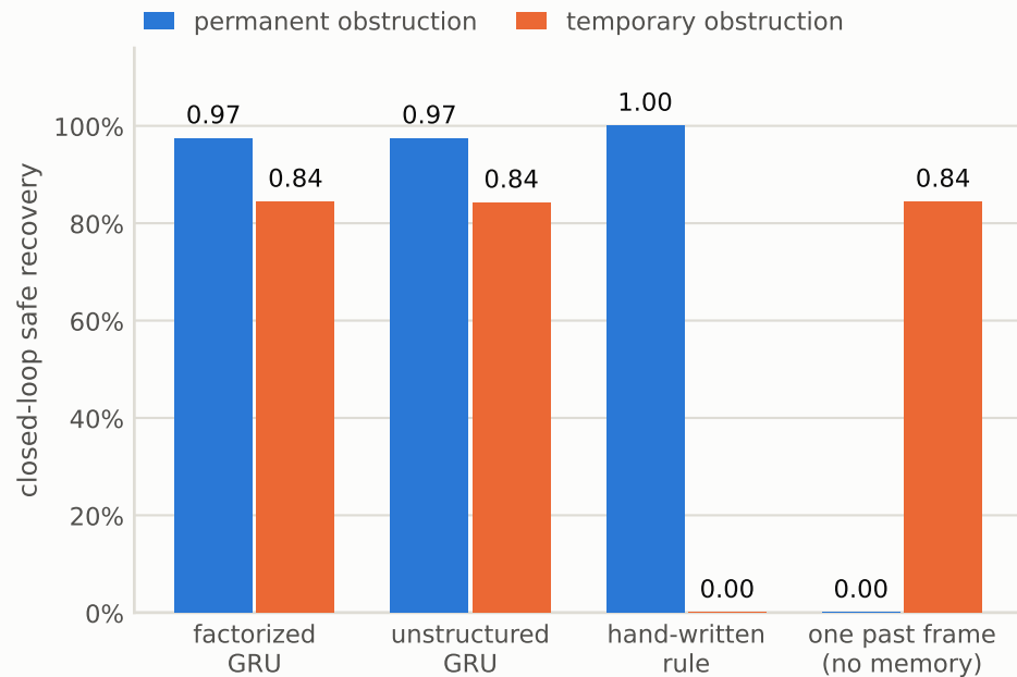
B. Both non-recurrent arms fail the confusion pair in opposite directions; both recurrent arms solve it
