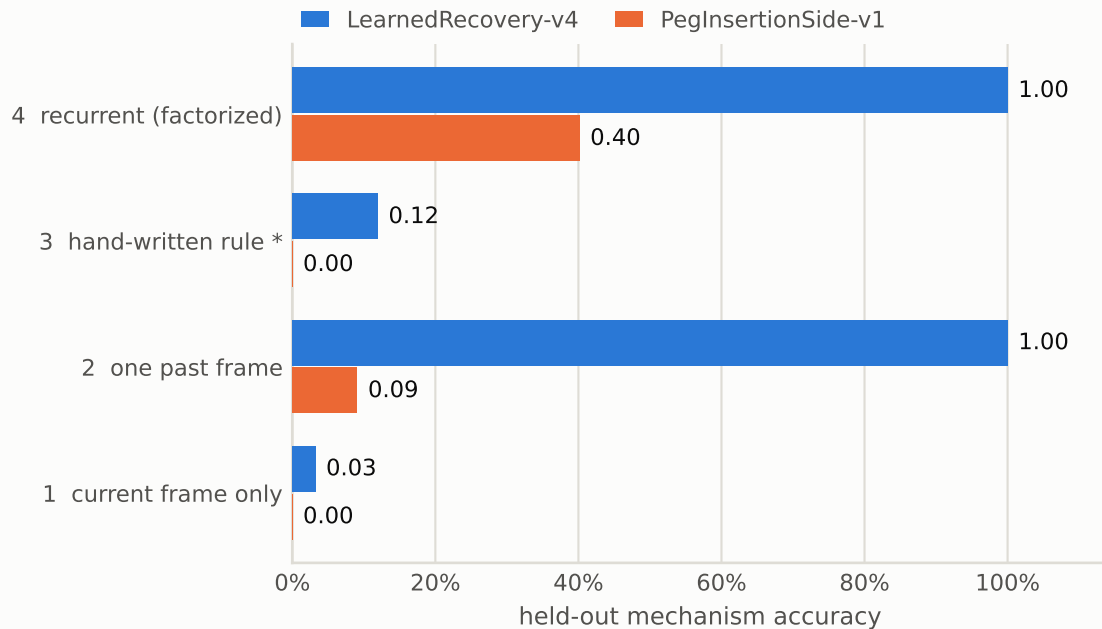
A. A lower rung matching rung 4 means the held-out mechanism is a shortcut, not a composition result
