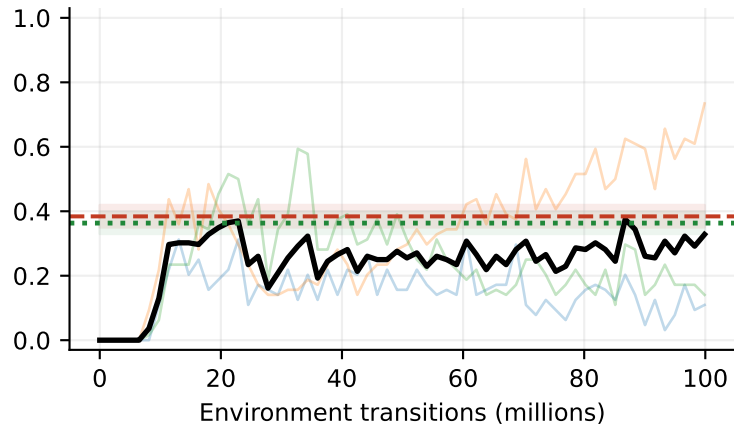
safe no intervention training
