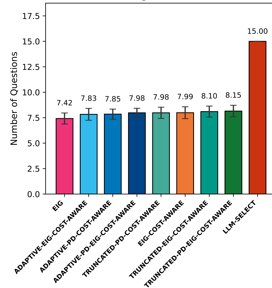
Average Questions
