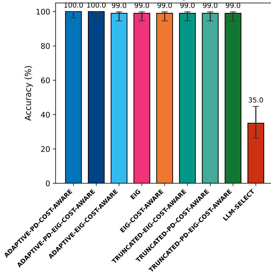
Accuracy
