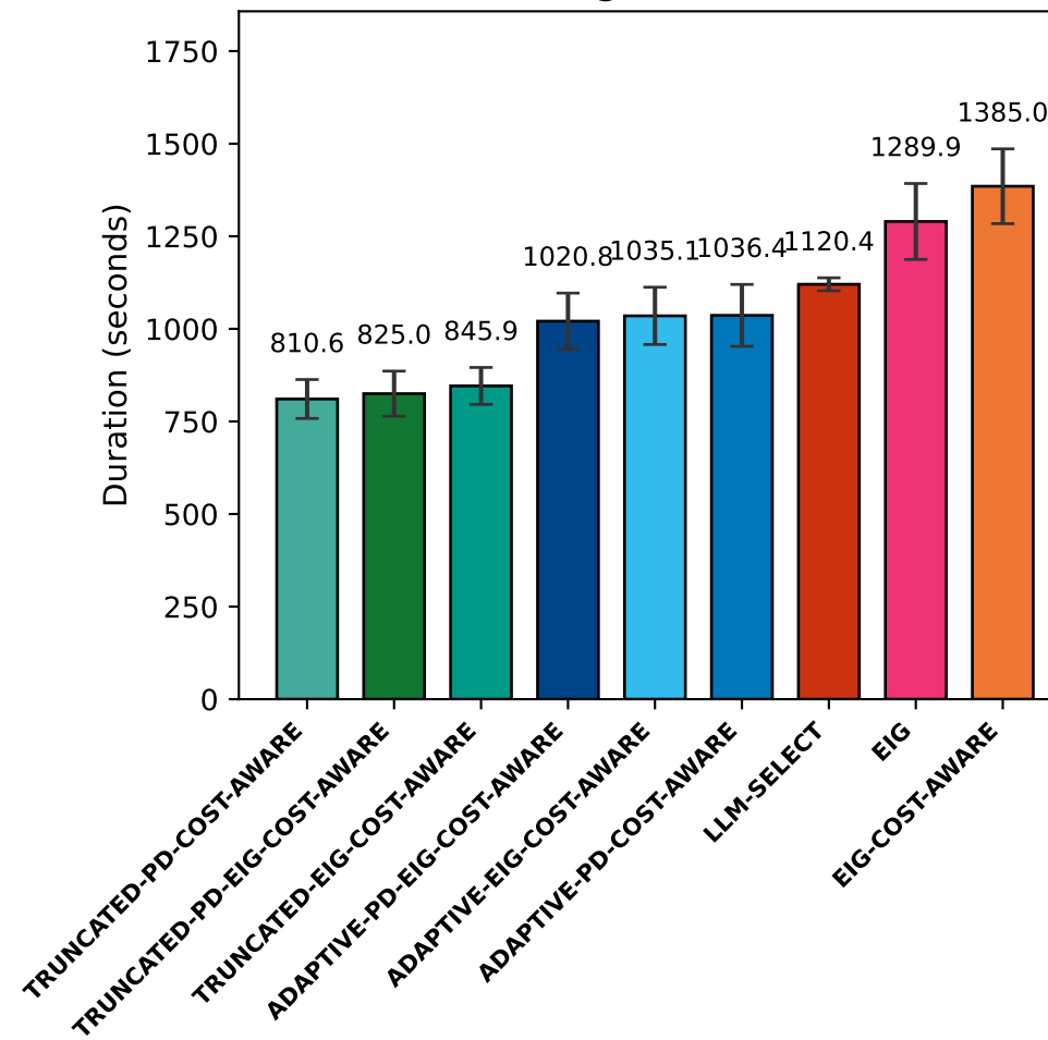
Average Duration
