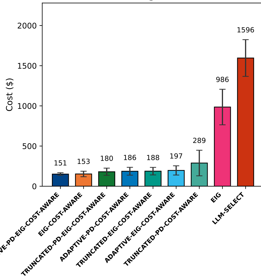
Average Cost
