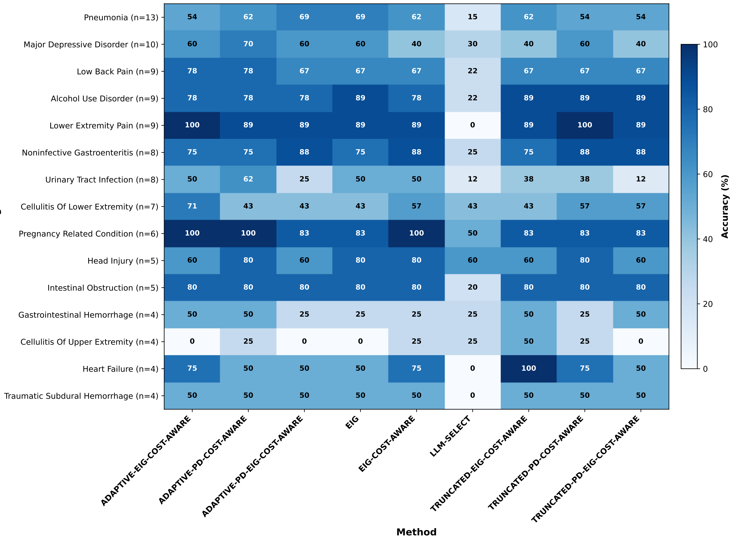
Accuracy by Diagnosis: I-NP (Informative Prior, No Pruning)
