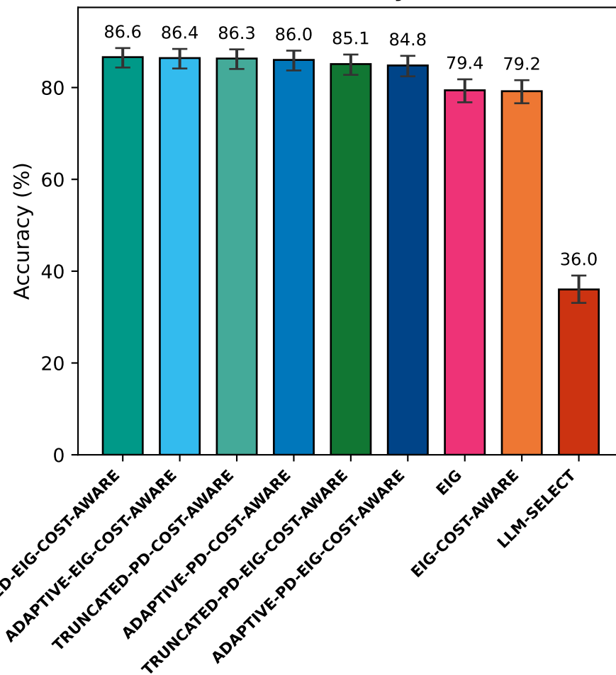
Accuracy
