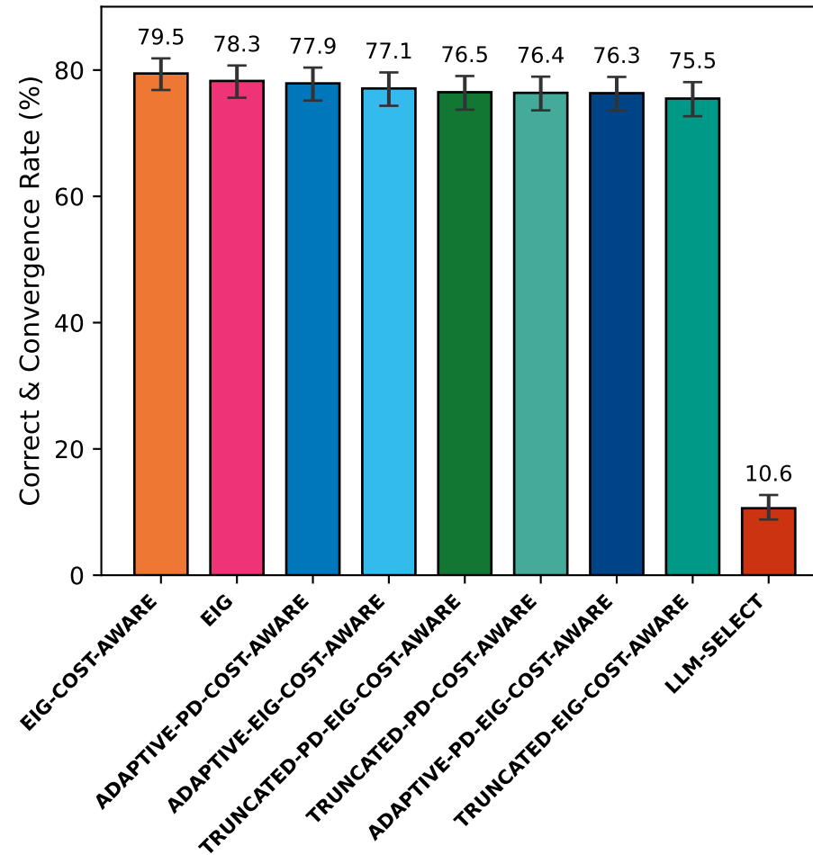
Correct & Convergence Rate
