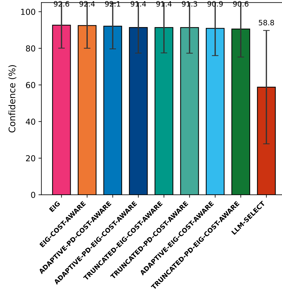
Average Final Confidence
