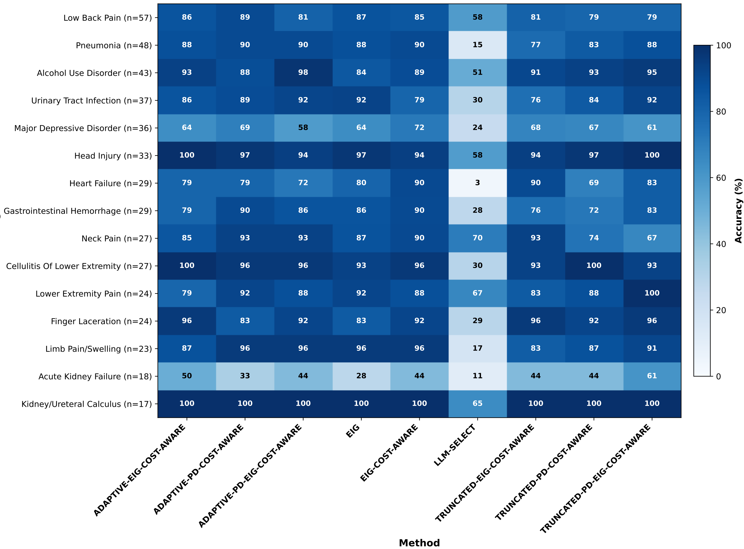
Accuracy by Diagnosis: I-P (Informative Prior, Pruning)
