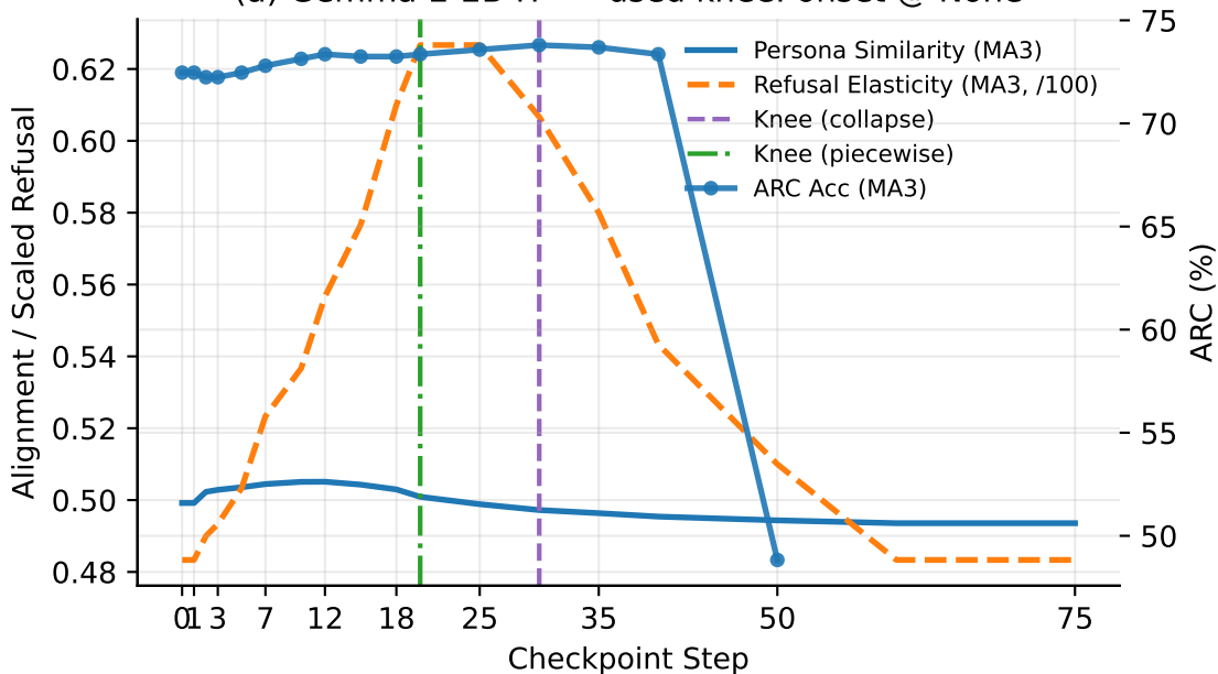
(a) Gemma-2-2B-IT — used knee: onset @ None
