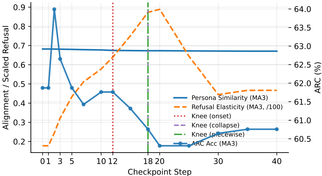
(c) Llama-3.2-3B-Instruct — used knee: piecewise @ 18
