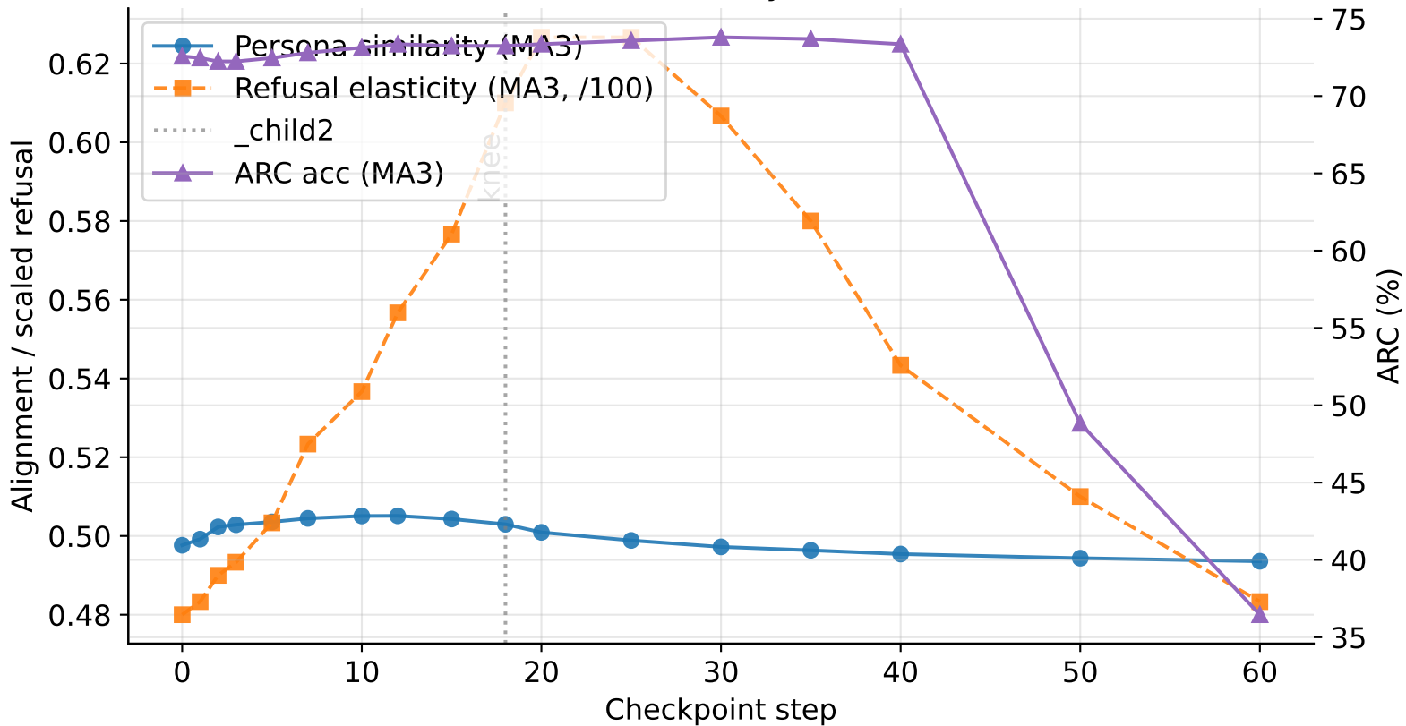
Gemma-2-2B-IT: identity/behavior vs ARC
