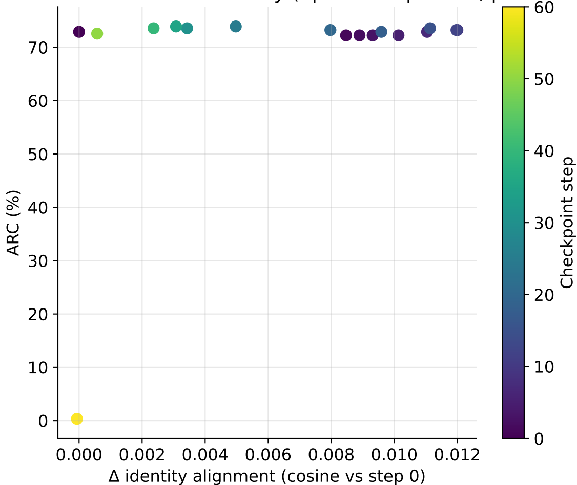
ma-2-2B-IT: ARC vs \Delta identity (Spearman \rho=0.04 , p=0.883 )
