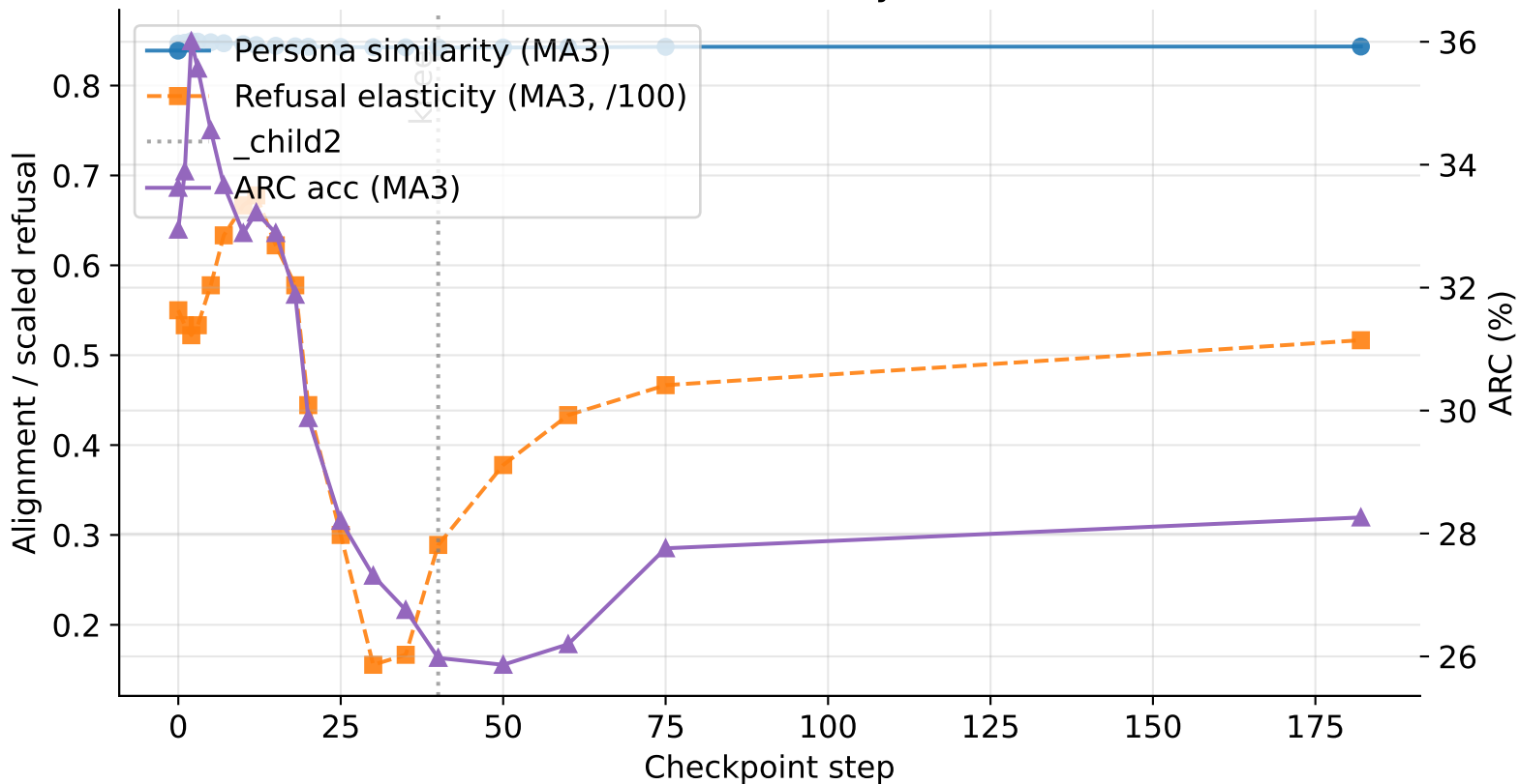
Llama-3.2-1B-Instruct: identity/behavior vs ARC
