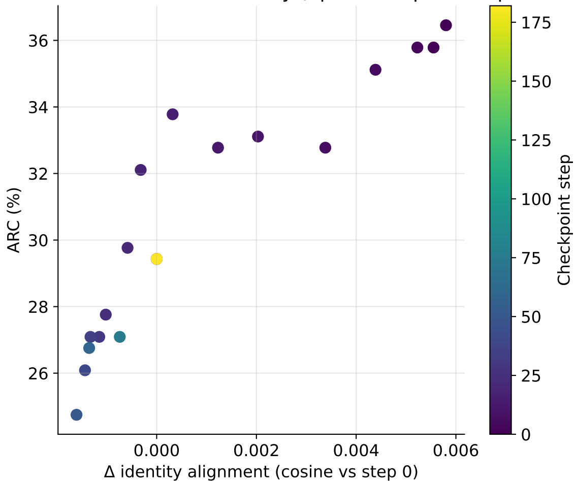
2-1B-Instruct: ARC vs \Delta identity (Spearman \rho=0.97 , p=1.77e-1 )
