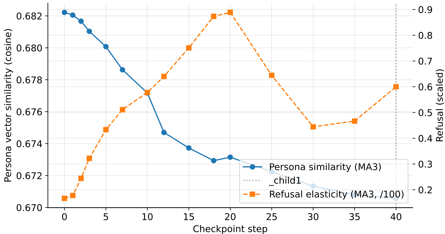
Llama-3.2-3B-Instruct: Phase-transition traces
