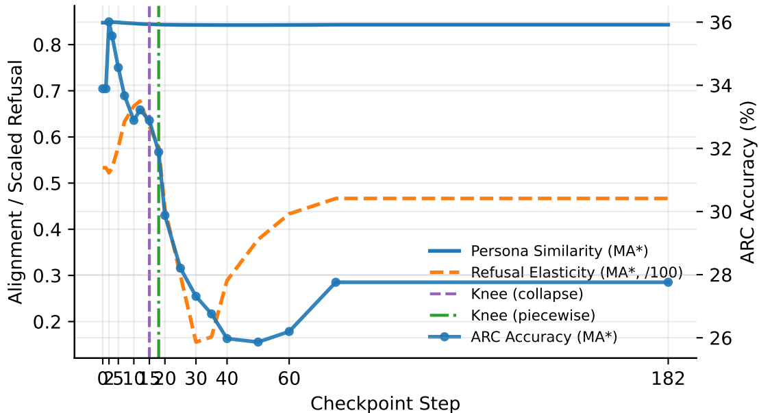
(b) Llama-3.2-1B-Instruct — used knee: collapse @ 15
