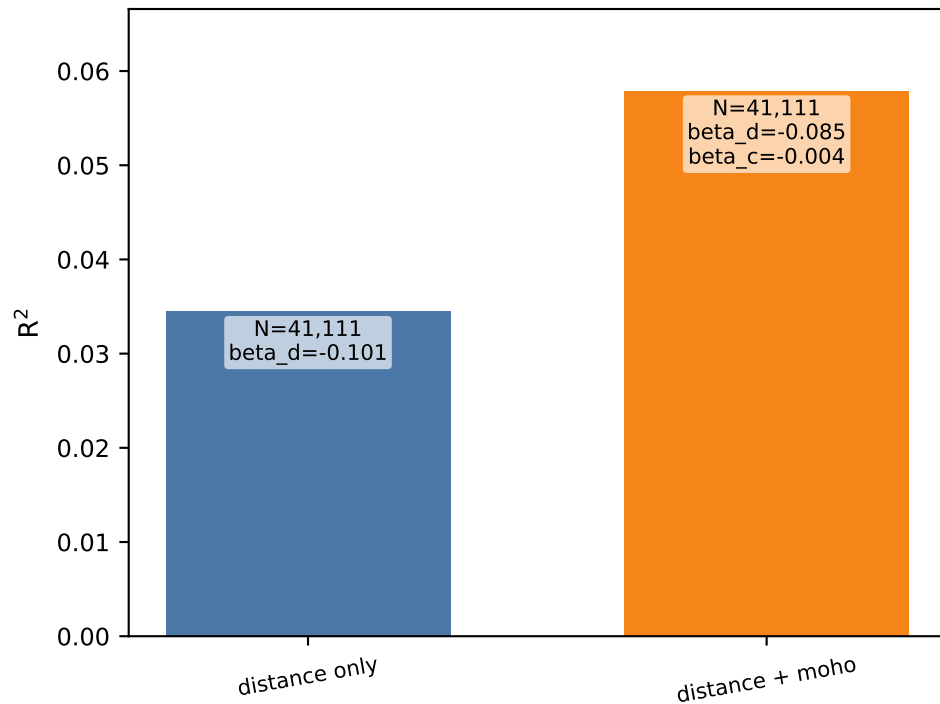
Continental domain: distance vs distance + Moho
