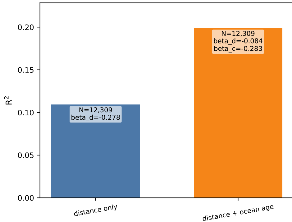
Oceanic domain: distance vs distance + ocean age
