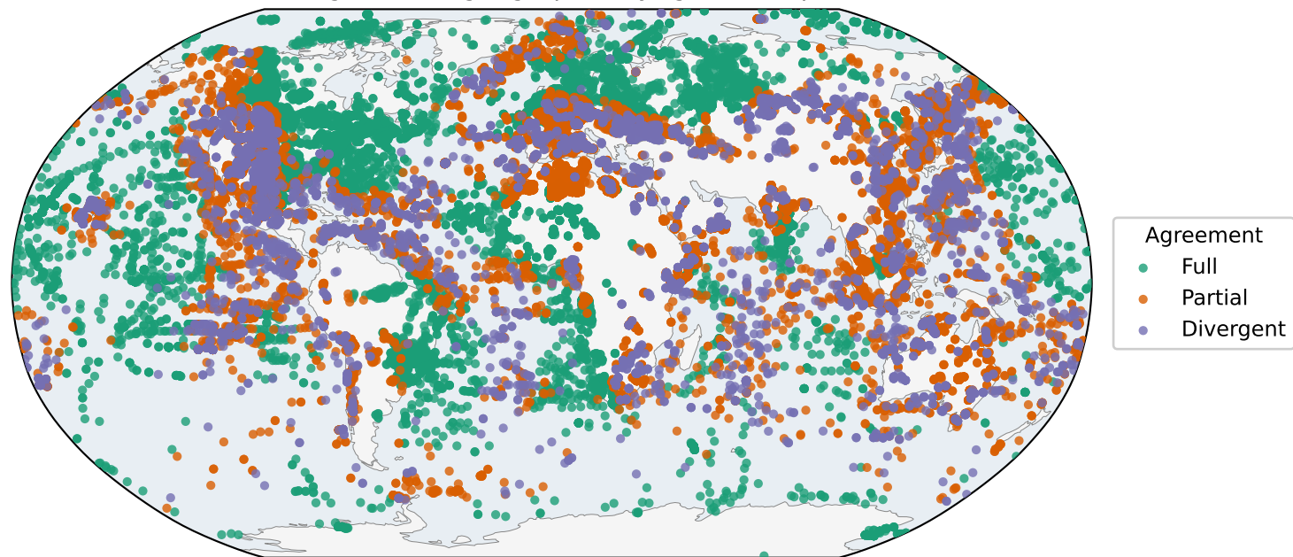
b Agreement geographically (global map)
